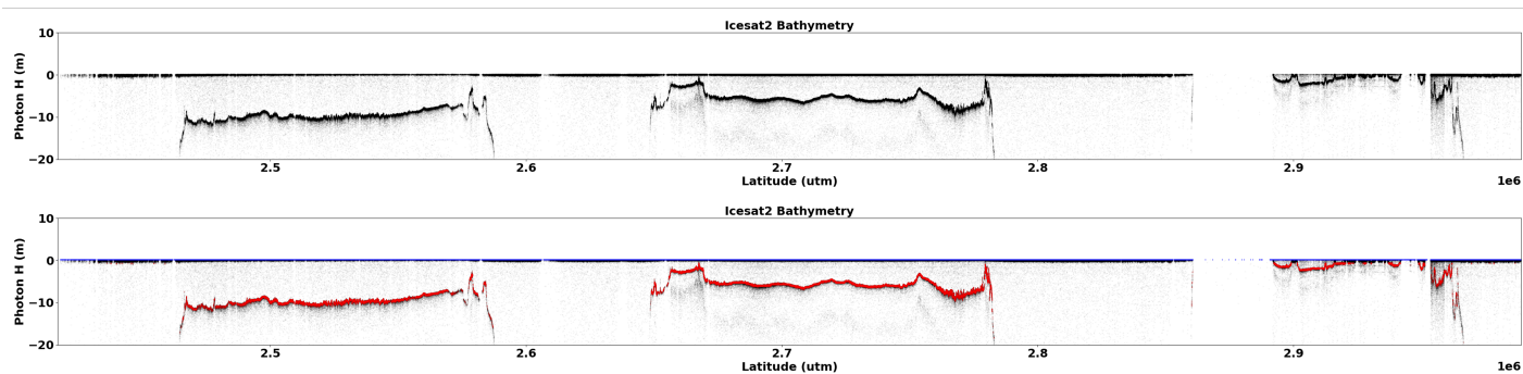
Fig. 3. ICESat-2 sub-aquatic photons. Top) Raw ICESat-2 data transformed to orthometric (EGM08) height. Bottom) Bathymetric classified photons (red) and surface classified photons (blue) from C-SHELPh. The algorithm is robust against a phenomenon known as ringing, whereby an artificial repeat of the surface is produced offset from the true surface, as visible below the red selected photons.
