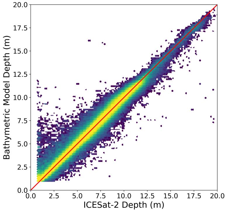
Fig. 6. Left: Relationship between ICESat-2 observed depth and modeled depth. There is no relationship between depth and residual error, with the majority of errors being small and occurring across all depths. Right: Summary statistics of the validation data for each of the three composite bathymetry maps.
