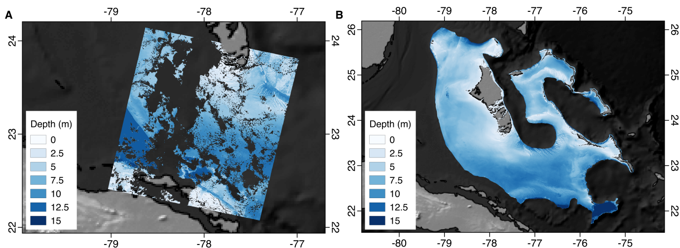
Fig. 4. A single bathymetric model generated from a single Landsat image (left) and a spatially continuous median composite for the Bahamas region (right) demonstrating a range of depths, with the deepest depths at the outer edge of the island complexes, such as at the Tongue of the Ocean.
