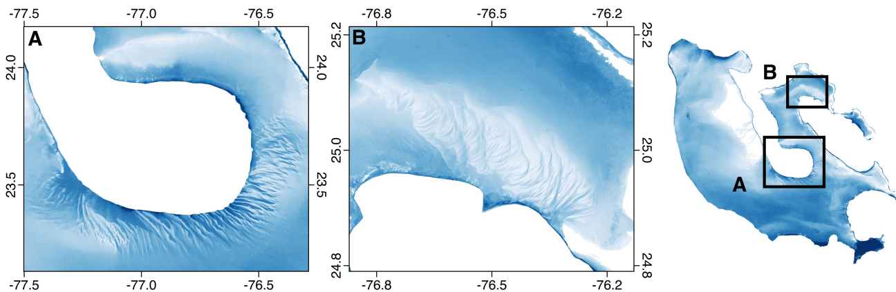
Fig. 5. Geomorphological features mapped with the bathymetry model. A) and B) show two distinct features with fine-scale variations in elevation.
