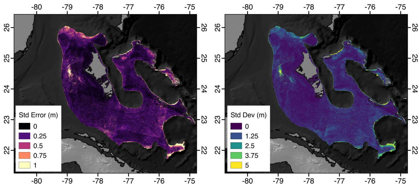
Fig. 7. Left: Standard error map of the region, detailing increased errors at increased depths. Right: Standard deviation map of the study site used to determine standard error. A region of inaccurately modeled deep bathymetry within the shallow bay at 24.5^{\circ} N, -79.3^{\circ} E, is visible.
