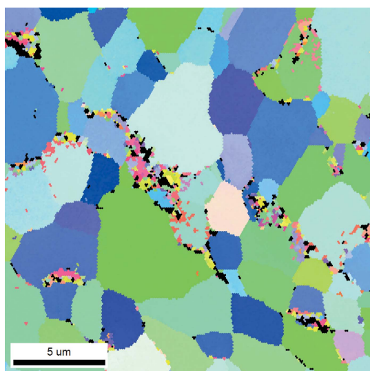
Figure 3 The EBSD inverse pole figure map obtained for the non-irradiated E110 sample.
