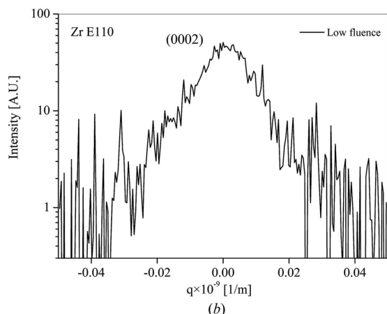
Figure 1 The intensity distribution at Bragg reflection 0002 with linear and logarithmic scales obtained for the sample E110 irradiated by the fluence 1.99 \times 10^{24} \text{ nm}^{-2} .
