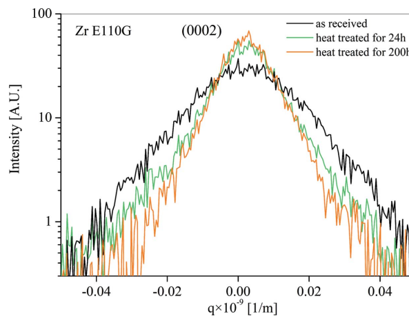
Figure 4 The intensity distributions of the 0002 reflection obtained for the as-received, heat treated for 24 h and heat treated for 200 h at 533 \pm 10 K samples.
