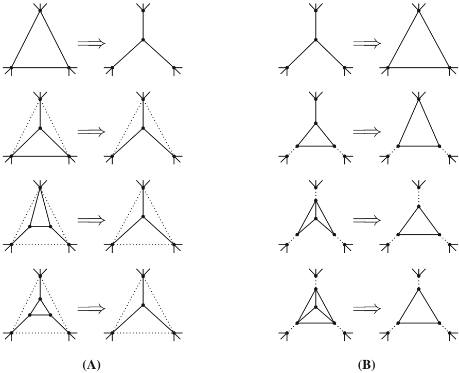
FIGURE 3. a Four types of simple \Delta -to- Y reduction, and b four types of simple Y -to- \Delta reduction, where the dotted lines denote edges that may or may not be present, and are not affected by the simple \Delta -to- Y and Y -to- \Delta reductions
