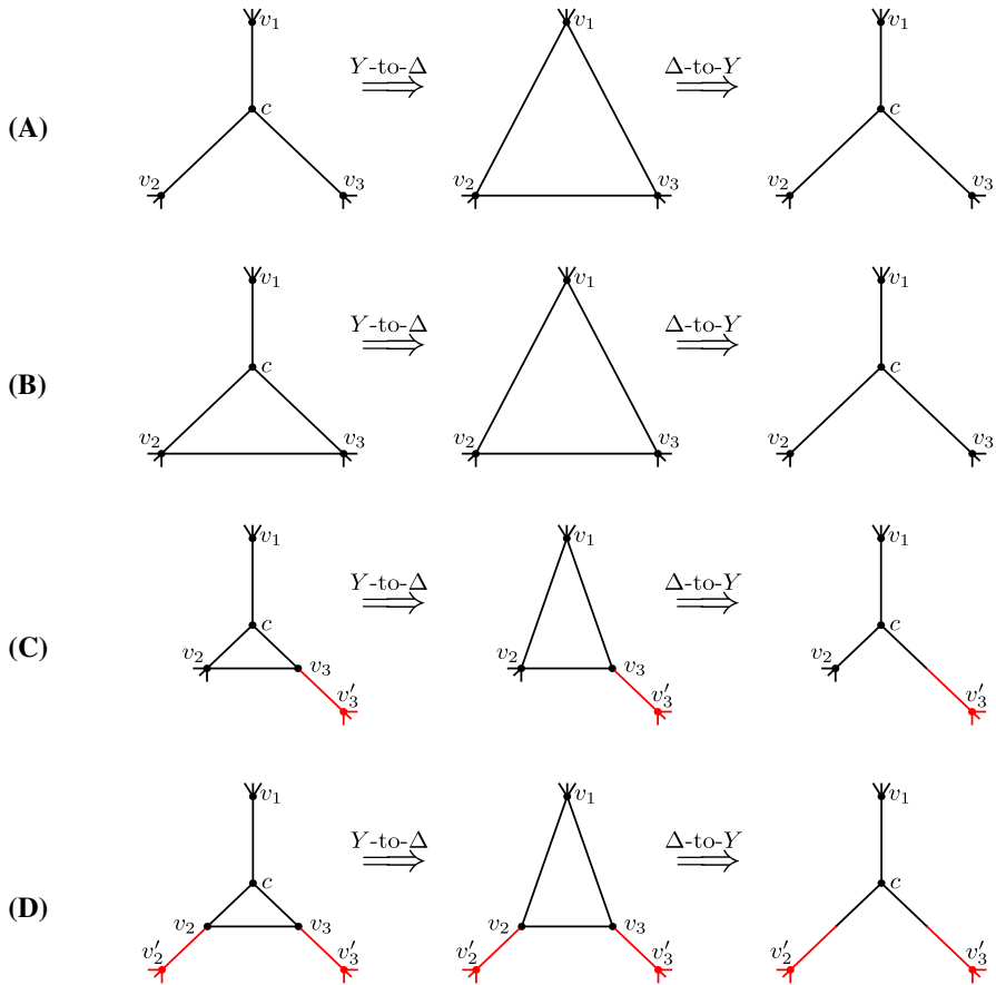
FIGURE 5. Reconstruction of reductions
