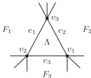
FIGURE 4. Face \Lambda and its neighbors
