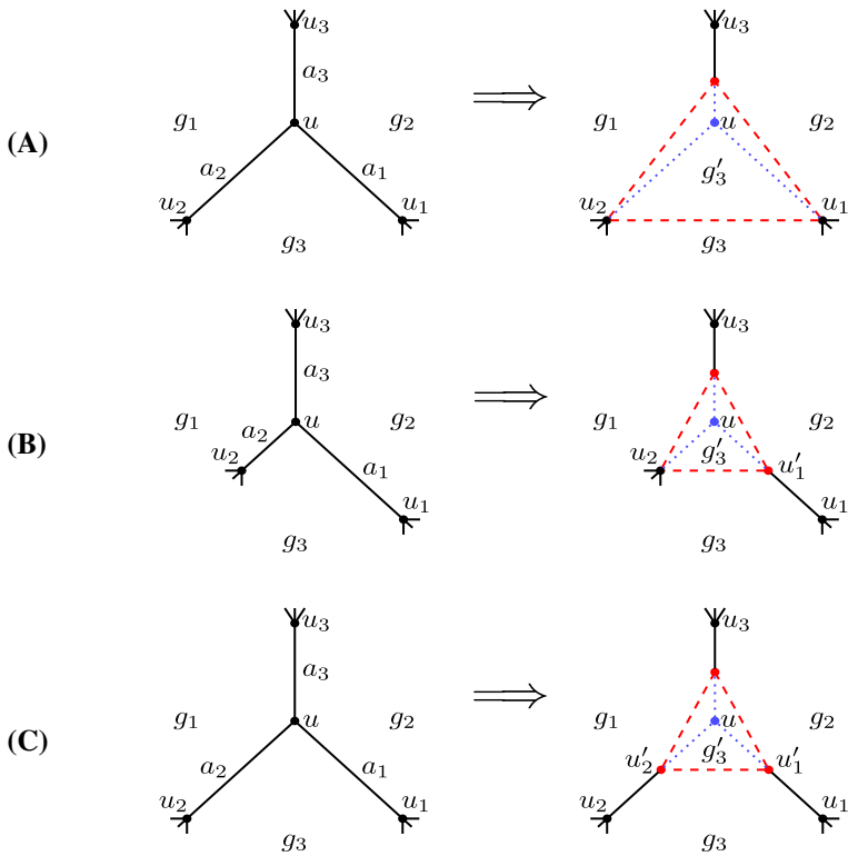
FIGURE 6. The dotted (blue) vertices and edges are removed and the dashed (red) vertices and edges are introduced in the new graph (Color figure online)
