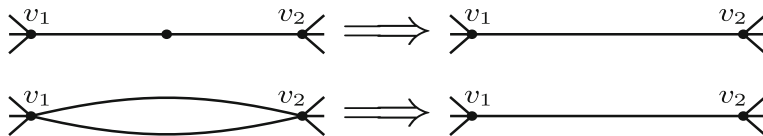
FIGURE 2. Examples of SP-reductions
