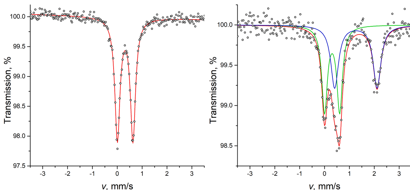
Fig. 8. Mössbauer spectra of the samples MS-2 (left) and XL-5 (right) measured at room temperature.
