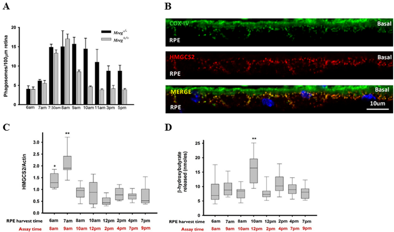
Figure 5. \beta -HB secretion is delayed coincident with slowed phagosome maturation in mouse RPE. A , loss of MREG leads to phagosome accumulation in the RPE. Phagosome numbers per 100 \mu\text{m} of RPE length in Mreg +/+ and Mreg -/- mice at different time points relative to lights on. Counts were done in duplicate on 10 individual areas per mouse in a total of 2 mice/4 eyes with analyst blind to the strain of mouse. The results are means \pm S.E. B , localization of HMGCS2 to mitochondria in mouse Mreg -/- RPE. Confocal micrographs of MREG -/- retinal sections immunostained for COXIV (green) and HMGCS2 (red) showing mitochondrial localization of HMGCS2 similar to WT. Nuclei are indicated in the merged image as blue. Note that the basolateral pattern of mitochondrial distribution closely resembling the WT. C , HMGCS2 protein levels in RPE explants utilized for \beta -HB release experiments in D . Cleared lysates were isolated immediately after the 2-h sample was collected, and Western blotting for HMGCS2 was performed as described under "Experimental procedures." **, p < 0.005. Plots are box-whisker plots showing median, with maximum and minimum range of the data for 12 eyes from 6 individual mice at each time point. D , \beta -HB is released from mouse RPE/choroid explants upon OS ingestion. Supernatant was collected from RPE/choroid explants, and \beta -HB levels were determined immediately. *, p < 0.05; **, p < 0.005. The plots are box-whisker plots showing median, with maximum and minimum range of the data for 12 eyes from 6 individual mice at each time point.
