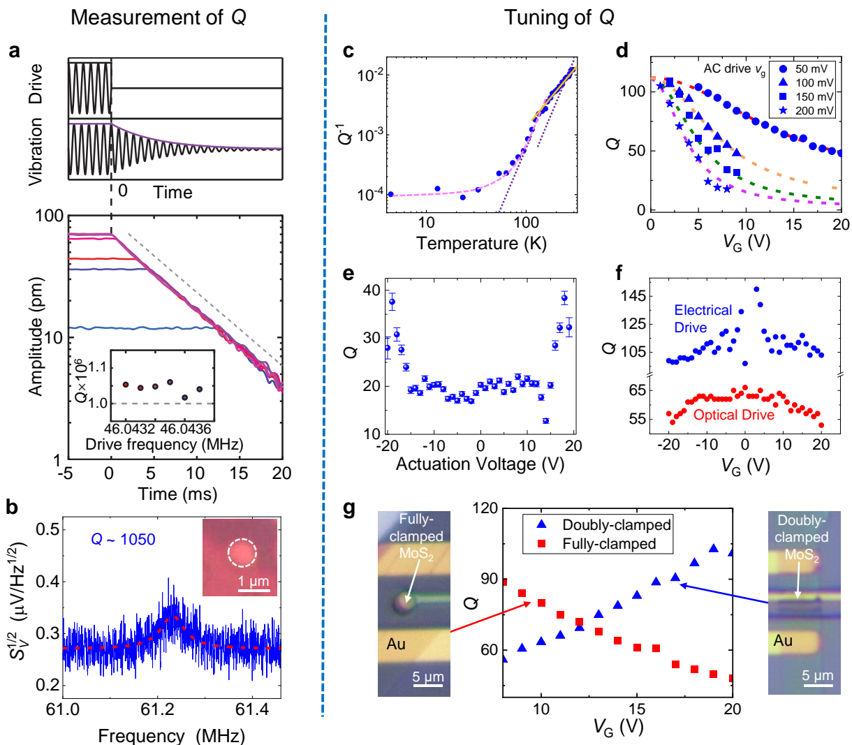
Figure 8.2. Q in 2D NEMS resonators. (a) A graphene resonators measured at 15 mK, showing Q exceeding 1 million. Reprinted in part with permission from ref 138. Copyright 2021 Springer Nature. (b) 2D MoS 2 resonators measured at room temperature, showing Q exceeding 1000. Reprinted in part with permission from ref 63. Copyright 2018 The Authors, some rights reserved; exclusive licensee AAAS. Distributed under a CC BY-NC 4.0 license http://creativecommons.org/licenses/by-nc/4.0/ . (c) Temperature dependence of Q for a 2D MoS 2 resonator. Reprinted in part with permission under a Creative Commons (CC-BY-NC-ND) License from ref 205. Copyright 2017 Nature Publishing Group. (d) Dependence of Q on AC gate voltage, for 2D MoS 2 NEMS resonators. Reprinted in part with permission from ref 208. Copyright 2022 American Chemical Society. (e) Q versus comb-drive actuation voltage for 2D MoS 2 resonator mounted on a comb-drive. Reprinted in part with permission from ref 183. Copyright 2021 Wiley-Blackwell. (f) Gate tuning of Q for MoS 2 resonators. Reprinted in part with permission from ref 63. Copyright 2018 The Authors, some rights reserved; exclusive licensee AAAS. Distributed under a CC BY-NC 4.0 license http://creativecommons.org/licenses/by-nc/4.0/ . (g) Different effect of tuning Q for fully-clamped and doubly-clamped 2D MoS 2 NEMS resonators using DC gate voltage. Reprinted in part with permission from ref 208. Copyright 2022 American Chemical Society.
