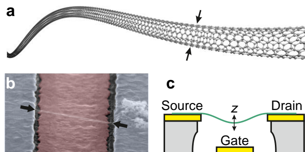
Figure 4.1. Structure of carbon nanotubes and typical device geometry of a nanotube resonator. (a) Illustration of the atomic lattice forming a nanotube. Individual carbon atoms are shown as spheres and carbon-carbon bonds as lines. The distance between the arrows is the tube diameter. (b) Colored scanning electron micrograph showing a nanotube over a trench. The gate electrode underneath the nanotube is shown in red. The arrows indicate the clamping points. Adapted with permission from ref 98. Copyright 2011 American Chemical Society. (c) Sketch of typical device geometry, with a nanotube (green) suspended freely between source and drain electrodes over a gate electrode and vibrating in z -direction. Metal electrodes are shown in yellow.
