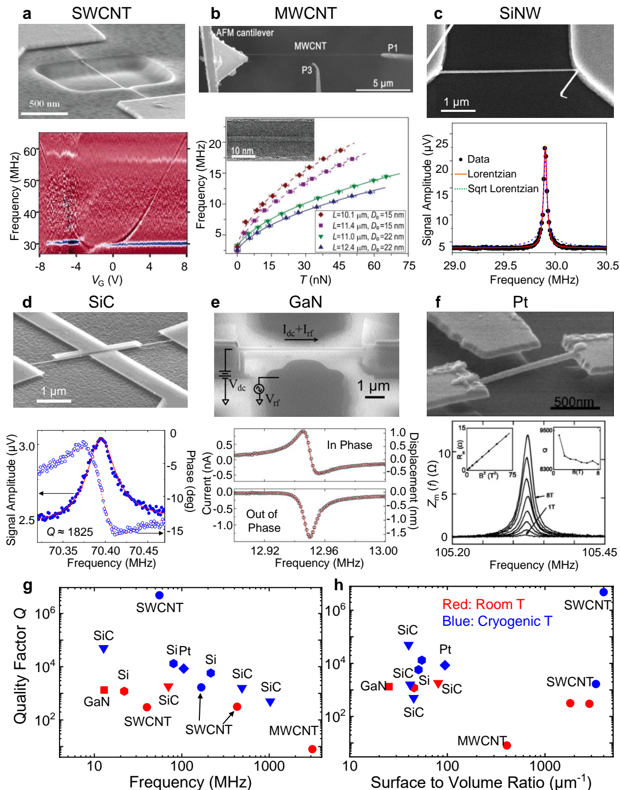
Figure 4.3. Examples of one-dimensional (1D) NEMS resonators, with scanning electron microscopy (SEM) images and representative resonance characteristics shown for (a) SWCNT, reprinted in part with permission from ref 198. Copyright 2006 American Chemical Society. (b) MWCNT, Reprinted in part with permission from ref 114. Copyright 2009 Wiley-VCH Verlag. (c) Si NW, reprinted in part with permission
