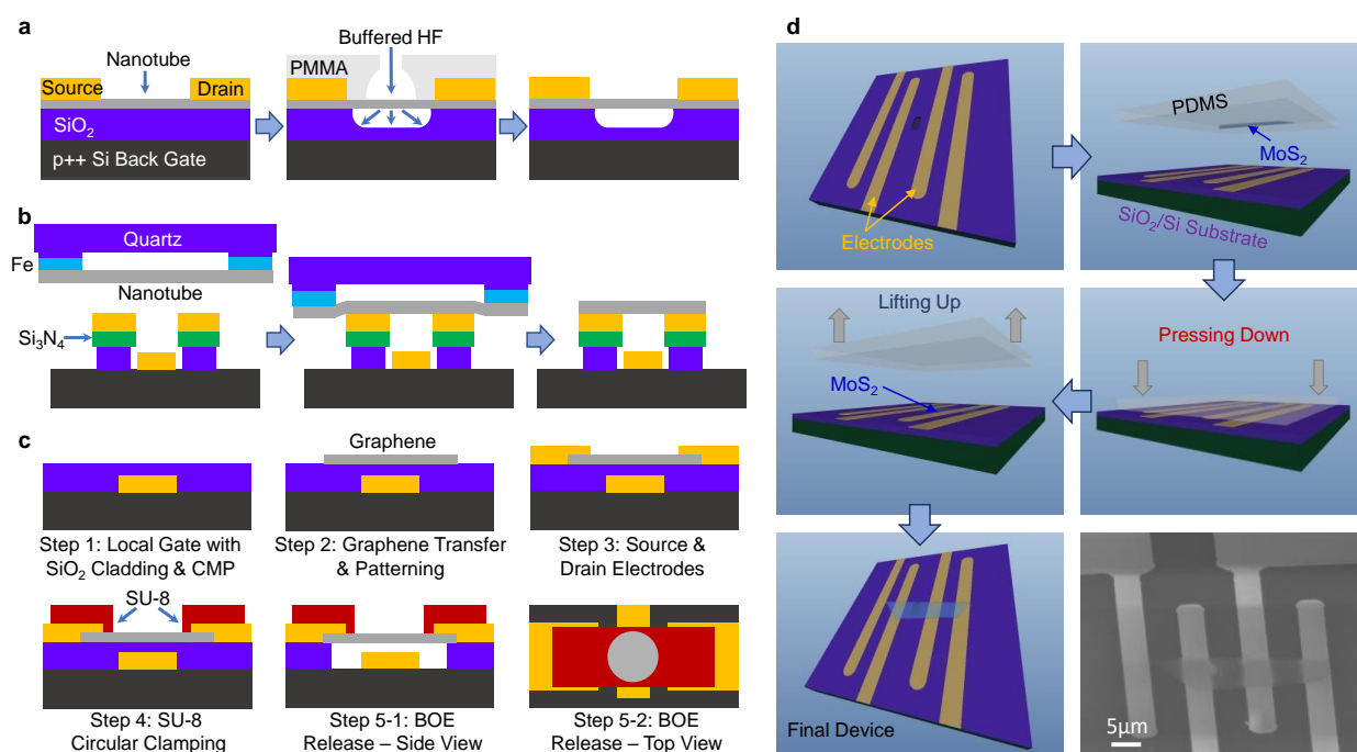
Figure 2.1. Schematic illustrations of fabrication processes for 1D and 2D NEMS resonators. (a) Suspending a nanotube by etching the sacrificial layer underneath using buffered HF etching. Reprinted in part with permission from ref 198 Copyright 2013 American Chemical Society. (b) One-step direct transfer of CNTs for NEMS resonators and other functional devices. Reprinted in part with permission from ref 49. Copyright 2010 American Chemical Society. (c) Etching of sacrificial layer underneath graphene, with SU-8 circularly clamping the graphene to form a circular resonator with a local gate electrode. Reprinted in part with permission from ref 58. Copyright 2013 American Physical Society. (d) Dry transfer of molybdenum disulfide (MoS 2 ) onto a substrate with predefined microtrenches and contact electrodes. Reprinted in part with permission from ref 61. Copyright 2014 AVS AMER INST PHYSICS.
