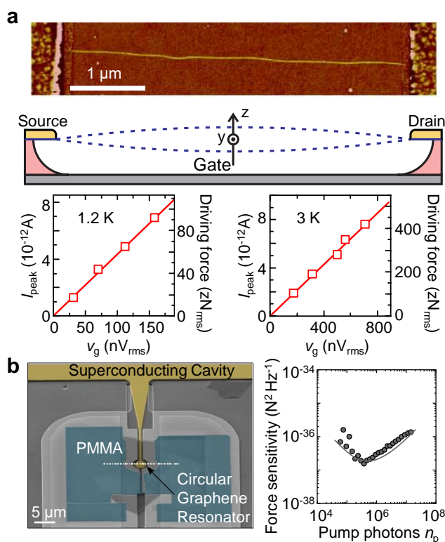
Figure 11.2. Force sensing applications of low-dimensional NEMS resonators. (a) Atomic force microscope (AFM) image of a 4 \mu\text{m} long nanotube, schematic of the device, and the corresponding force sensing experimental results showing zN force sensing at 1.2 K and 3K. Reprinted in part with permission from ref 91. Copyright 2013 Nature Publishing Group. (b) False-colored image of a multilayer graphene resonator and the force sensitivity under different numbers of pump photons. Reprinted in part with permission under a Creative Commons (CC BY) License from ref 77. Copyright 2016 Nature Publishing Group.
