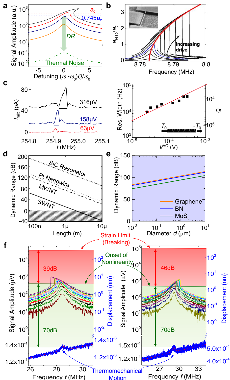
Figure 9.1. Nonlinearity and dynamic range in 1D and 2D NEMS resonators. (a) Definition of dynamic range in a NEMS resonator, from thermomechanical resonance to onset of nonlinearity as vibration amplitude increases. Reprinted in part with permission from ref 218. Copyright 2014 American Institute of Physics. (b) Resonance spectra of the doubly-clamped SiC nanowire resonator with increasing drive,
