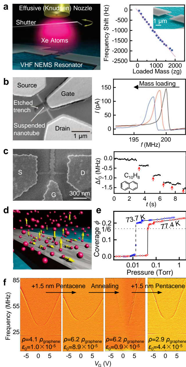
Figure 11.1. Mass sensing applications using NEMS resonators. (a) Schematic illustration of Xe atom mass sensing using a SiC nanowire resonator, and the measured frequency response to mass loading, showing zg-level mass sensing. Reprinted in part with permission from ref 247. Copyright 2011 American Chemical Society. (b) SEM image and resonance curve during adsorption for a CNT resonator. Reprinted in part with permission from ref 71. Copyright 2008 American Chemical Society. (c) SEM image and mass sensing data for a CNT resonator, showing down to 1.7 yoctogram resolution. Reprinted in part with permission from ref 250. Copyright 2012 Nature Publishing Group. (d) Schematic illustration of fluctuation of Xe atoms (including adsorption, desorption, and surface diffusion) on a SiC nanowire resonator. Reprinted in part with permission from ref 247. Copyright 2011 American Chemical Society. (e) Low-dimensional phase transition of Kr atoms adsorbed on the surface of a CNT resonator, detected by monitoring the resonance frequency. Reprinted in part with permission from ref 42. Copyright 2010 American Association for the Advancement of Science. (f) Mass sensing behavior of graphene resonator. Reprinted in part with permission from ref 57. Copyright 2009 Nature Publishing Group.
