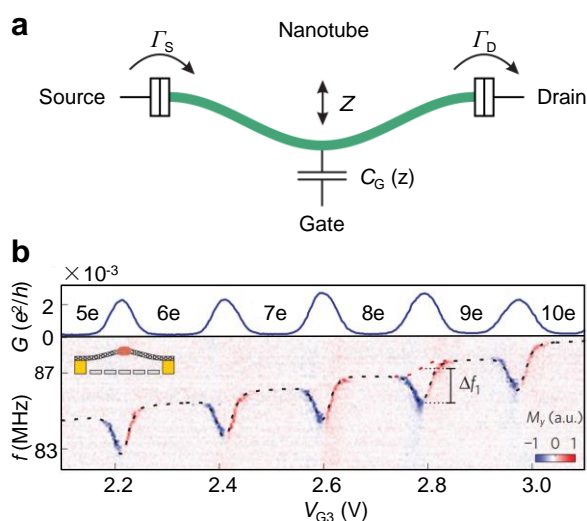
Figure 12.3. CNT resonator as a quantum dot. (a) Sketch of a carbon nanotube coupled to source and drain leads with charge transport rates \Gamma_{S,D} . The total electrical charge of the nanotube can be tuned capacitively by a gate voltage. The nanotube-gate capacitance C_G(z) depends on the nanotube displacement z . (b) Electrical conductance and mechanical resonance frequency as a function of the gate voltage measured at a temperature of 16 K. Reprinted in part with permission from ref 272. Copyright 2012 American Physical Society.
