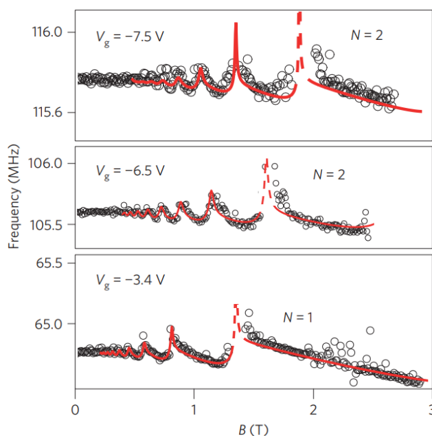
Figure 12.4. Mechanical resonant frequency in a graphene resonator as functions of the applied magnetic fields at different V_g , and corresponding fits (red curves). Reprinted in part with permission from ref 282. Copyright 2016 Nature Publishing Group.
