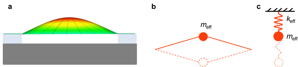
Figure 7.1. Mechanical model of a 2D resonator. (a) Schematic illustration (side view) of a fully-clamped 2D NEMS resonator in its fundamental mode. (b) A simplified version of the resonator showing the vibration of the effective mass. (c) The lumped parameter model of the resonator in a spring-mass system.
