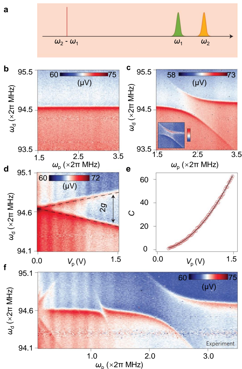
Figure 10.4. Parametric coupling in NEMS resonators. (a) Illustration of a red-detuned pump alongside the two coupled modes in the frequency domain. (b,c) The response of mode 1 as a function of the red-pump detuning when V_p = 0\text{V} (b) and V_p = 1.5\text{V} (c) in a graphene drumhead resonator. For non-zero pump amplitudes, mode 1 is seen to split in the vicinity of \omega_p \approx |\omega_1 - \omega_2| . Inset, the response detected at \omega_d + \omega_p . Energy transfer to the second mode is seen when \omega_d + \omega_p \approx \omega_2 . (d) Response of mode 1 at fine intervals of the pump voltage. (e) Cooperativity, a figure of merit that quantifies the magnitude of intermodal coupling, versus pump amplitudes. The solid line is a quadratic fit of the data (circles) to the equation C = \alpha V_p^2 . (f) Higher-order parametric coupling in NEMS resonators: mode 1 response as a function of the pump detuning over a larger frequency range in a graphene drumhead resonator. Apart from normal mode splitting at \omega_p \approx \Delta\omega = |\omega_1 - \omega_2| , an extra splitting at \omega_p \approx (\Delta\omega)/2 can be seen, suggesting the onset of higher-order intermodal coupling. (a-f) are reprinted in part from Ref. 227. Copyright 2016 Nature Publishing Group.
