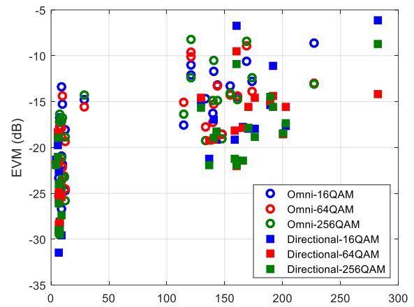
(b) EVM vs. RMS delay spread in IMC Hall
