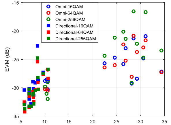
(a) EVM vs. RMS delay spread in DAL
