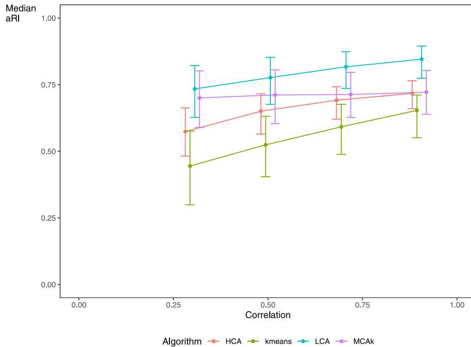
Fig. 1. Simulated dataset of patients with two or more conditions in 3 clusters, within cluster disease prevalence approximately 15%, noise approximately 0.5%, overlap of diseases between clusters: examining the effect of varying correlation of diseases within a cluster. Error bars show interquartile range (IQR).
