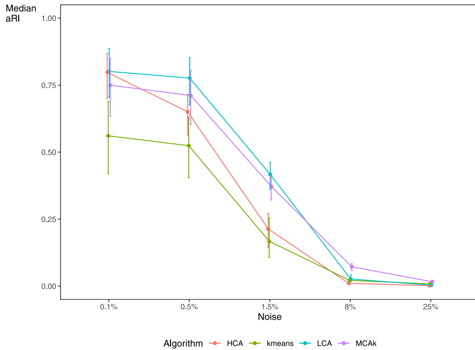
Fig. 2. Simulated dataset of patients with two or more conditions in 3 clusters, within cluster disease prevalence approximately 15%, correlation = 0.5, overlap of diseases between clusters: examining the effect of varying the amount of noise.
