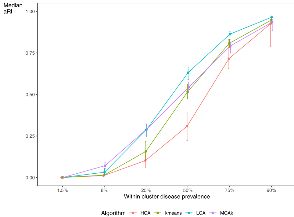
Fig. 3. Simulated dataset of patients with two or more conditions in 3 clusters, noise approximately 4%, correlation = 0.5, overlap of diseases between clusters: examining the effect of varying within cluster prevalence of disease.
