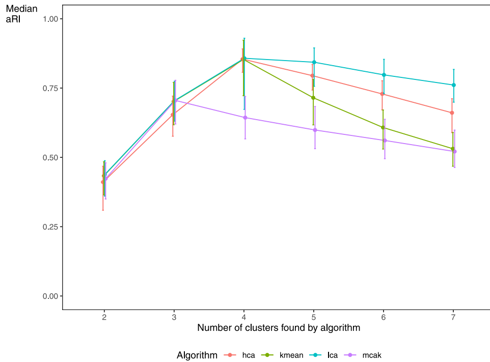
Fig. 4. Simulated dataset of patients with two or more conditions in 4 clusters, within cluster disease prevalence approximately 24%, noise approximately 0.5%, correlation = 0.5, overlap of diseases between clusters: examining the effect of varying the number of clusters algorithm is asked to find.
