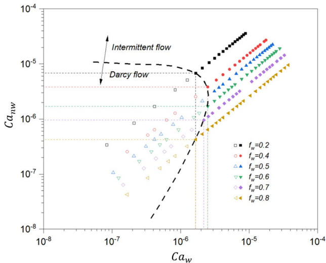
Figure 2. The phase diagram of the transition from Darcy flow (empty symbols) to intermittent flow (filled symbols) as a function of nonwetting phase capillary number Ca_{nw}^i , and wetting phase capillary number Ca_w^i ; the dashed line is the predicted threshold using Equations 7 and 8.
