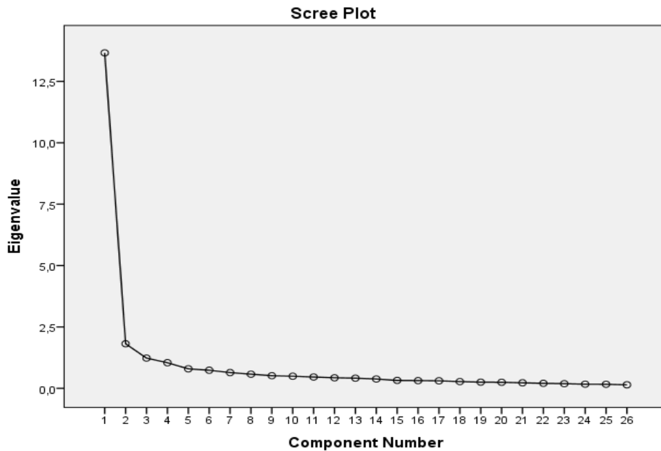
Graph 1. Scree plot
