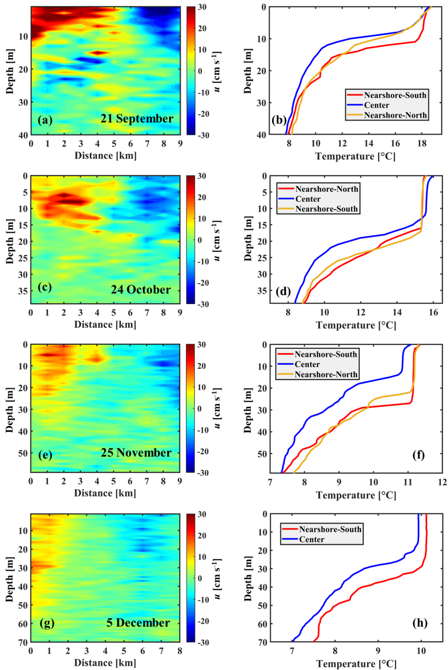
Figure 13. Left column: contour plots of the measured horizontal velocity along Transect T2 (for location, see Fig. 1b). Right column: measured temperature profiles at the locations marked by corresponding coloured triangles above panels in the left column: (a) and (b) 21 September 2019, (c) and (d) 24 October 2019, (e) and (f) 25 November 2019, (g) and (h) 5 December 2019. Note that all panels in the left column are plotted with the same range to highlight the seasonal change; the range of the x axis in the right column changes with time. Colour bars show the range of horizontal velocities.
