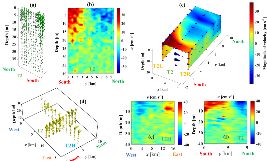
Figure 8. Measured current velocity field for sampling points along the selected transects (T) shown in Fig. 1b for (a) current vector profiles and (b) contour plot for 20 September 2019, (c) vectors (black arrows) and contours (see colour bar legend) for 21 September 2019, (d) current vector profiles, (e, f) contour plots for 22 September 2019. The coordinates of sampling points in T2 are the same in (a)–(d) and (f). The colour bars indicate horizontal velocity in centimetres per second. Positive velocities are pointing eastward for transect T2 and northward for transect T2H. Colour bars give the range of the horizontal velocity.
