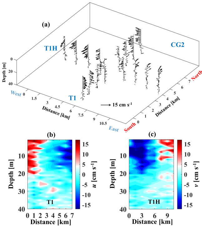
Figure 10. Field campaign of 25 October 2019: (a) current velocity field of CG2 shown as vector profiles at the different stations along transects T1 and T1H. (b, c) Contour plots of the horizontal components of velocity field, u (along T1) and v (along T1H). The origin of the x axis is in the south for T1 and in the west for TH1. The colour bars indicate horizontal velocity in centimetres per second. Positive velocities are pointing eastward for transects T1, T2, and T3 and northward for transect T1H. For transect location, see Fig. 1b.
