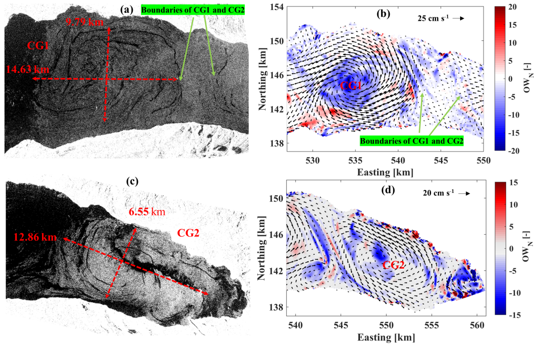
Figure 4. (a, c) SAR images (Sentinel-1) indicating two cyclonic gyres (CGs) in the eastern part of Lake Geneva for (a) CG1 (21 July 2018) and (c) CG2 (12 October 2018). Dashed red lines: major gyre axes and their dimensions. (b, d) Corresponding modelled surface velocity fields (small black arrows) and OW_N parameter values (colours). Strong negative OW_N parameter values (blue) indicate the location of core zones of large-scale gyres and mesoscale eddies. The colour bars give the range of the OW_N values.
