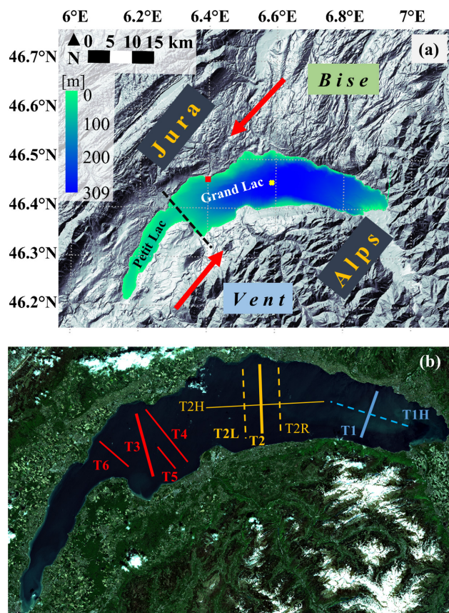
Figure 1. (a) Lake Geneva and surrounding topography, adapted from a public domain satellite image ( https://worldwind.arc.nasa.gov/ , last access: 29 October 2022) and bathymetry data from https://www.swisstopo.admin.ch/ (last access: 29 October 2022). The colour bar indicates the water depth. SHL2 (yellow cross) is a long-term CIPEL monitoring station where data on physical and biological parameters are measured. The red square shows the location of the EPFL Buchillon meteorological station (100 m offshore). The dashed black line approximately delimits the two basins of Lake Geneva called the Petit Lac (west) and the Grand Lac (east). The thick red arrows indicate the direction of the two strong dominant winds, called the Bise (coming from the north-east) and the Vent (coming from the south-west). (b) A schematic view of transects (T) selected for the different field campaigns in this study (for details, see text and Table S1 in the Supplement). The background satellite image is taken from Sentinel-1A.
