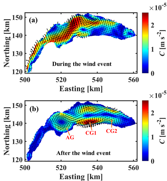
Figure 14. (a) Contribution of Coriolis term C (strength as indicated by colour contours and orientation by arrows) to the vertically (upper 5 m of the water column) and temporally (65 h) averaged horizontal-momentum equation (Eq. 6): (a) during and (b) after the Bise event that occurred in September 2019. After the wind event, convergence can be seen at gyre AG and divergence in the CG1 gyre area.
