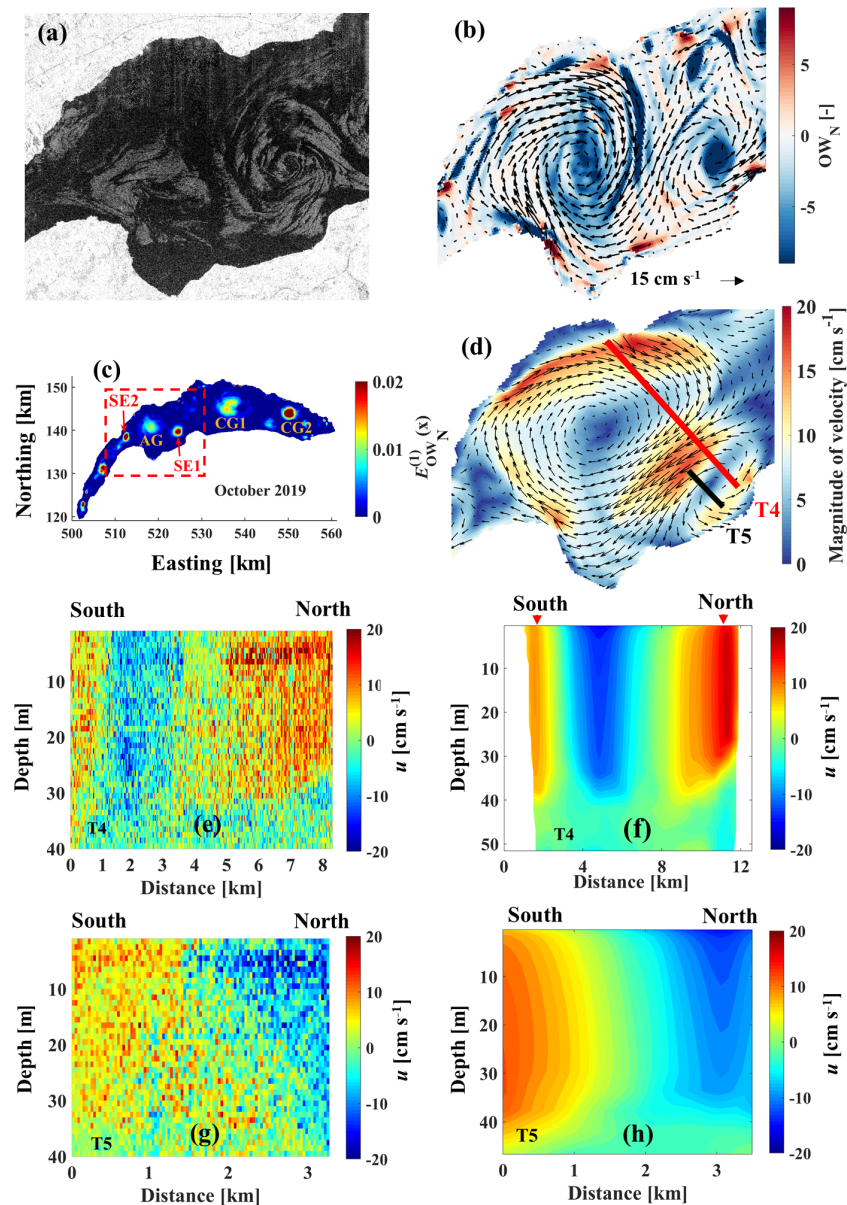
Figure 11. Evidence for the existence of submesoscale eddy 1 (SE1). (a) Remote sensing evidence (SAR images, Sentinel-1) of SE1 for 27 October 2019. (b) Corresponding modelled surface velocity fields (small black arrows show sense of rotation) and OW_N values shown by colours. (c) First EOF mode of OW_N for October 2019 showing large gyres AG1, CG1, and CG2 and small eddies SE1 and SE2. (d) Modelled surface velocity fields for 19 October 2020 and selected transect locations (T4, T5). (e) Measured horizontal current velocity profile along T4. (f) Corresponding modelled horizontal velocity along T4. (g) Measured horizontal current velocity profile along T5. (h) Corresponding modelled horizontal velocity along T5. Dashed-red-lined rectangle in (c) indicates the location of zoom panels (a), (b), and (d). Colour bars give the range of the parameters in the panels. Positive horizontal velocity points eastward.
