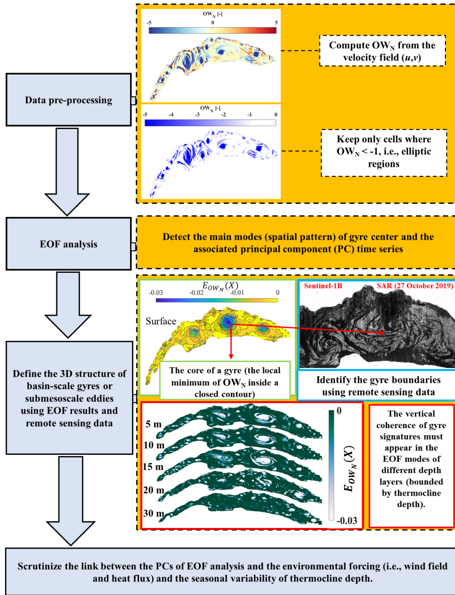
Figure 2. Flowchart of the proposed procedure showing the four steps (grey boxes) for detecting basin-scale gyres and eddies applied to Lake Geneva. Modelling results for the October 2019 Bise wind event, together with the corresponding SAR image, are used to highlight certain steps of the proposed procedure. For details, see text.
