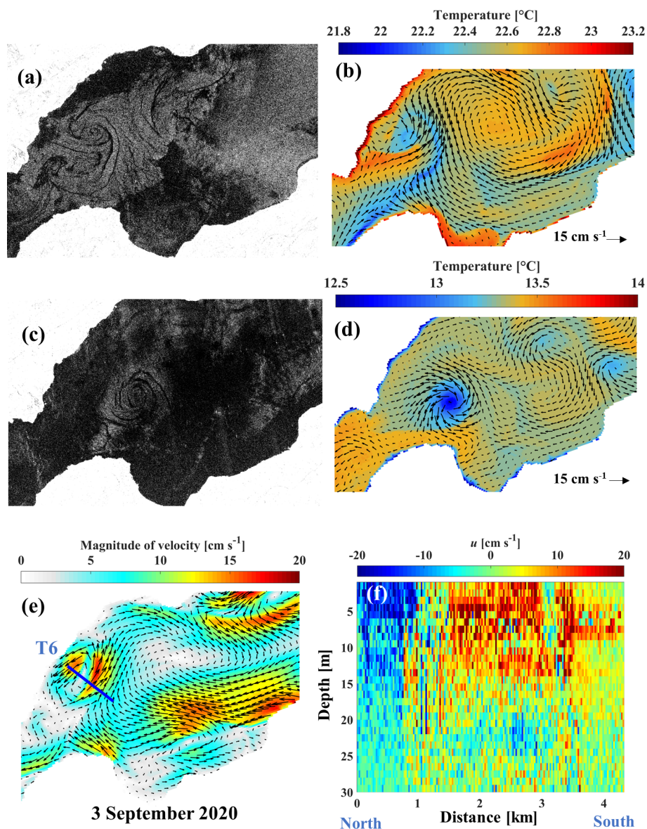
Figure 12. Evidence for the existence of submesoscale eddy 2 (SE2). (a) Remote sensing evidence (SAR image, Sentinel-1) of SE2 for 19 August 2018. (b) Corresponding modelled surface velocity fields (small black arrows) and temperatures shown by colours. (c) SAR image of SE2 for 7 November 2018. (d) Corresponding modelled surface velocity and temperature fields for 7 November 2018. (e) Modelled surface velocity and selected transect (T6) for the field campaign of 3 September 2020. (f) Measured horizontal current velocity along T6. For location of these panels, see Fig. 11c. Colour bars give the range of the parameters in the panels. Positive horizontal velocity points eastward.
