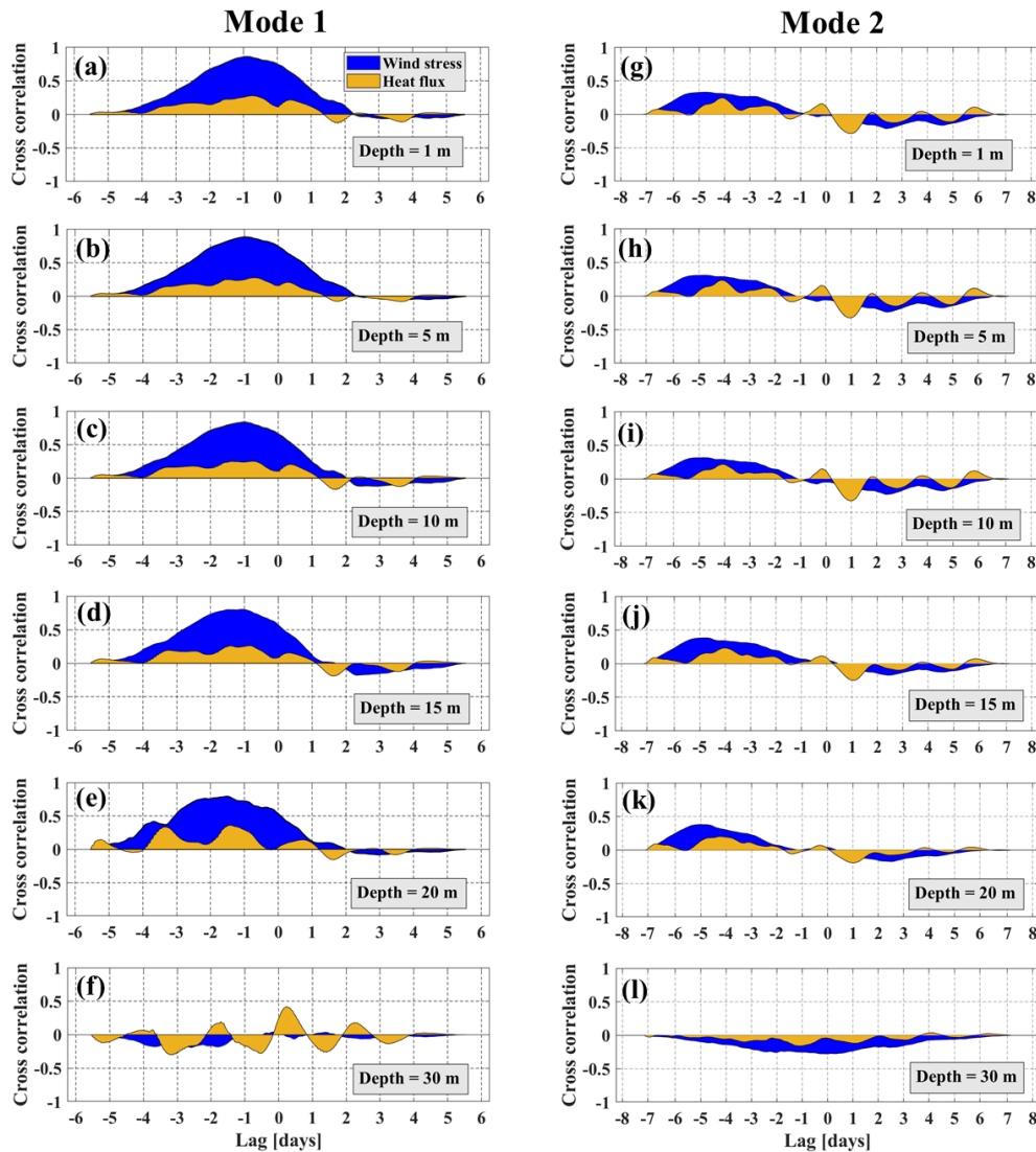
Figure 6. (a–f) Lagged cross-correlation of the principal component time series of the total wind stress ( \varphi_w^{(1)}(t) ) and the net upward heat flux ( \varphi_{HF}^{(1)}(t) ) with the principal component time series of the OW_N parameter associated with the first spatial mode ( P_{OW_N}^{(1)}(t) ) in different depth layers. (g–l) Lagged cross-correlation of the principal component time series of the total wind stress ( \varphi_w^{(1)}(t) ) and the net upward heat flux ( \varphi_{HF}^{(1)}(t) ) with the principal component time series of the OW_N parameter associated with the second spatial mode ( P_{OW_N}^{(2)}(t) ) in different depth layers. Wind stress and heat flux are defined in the colour legend in panel (a).
