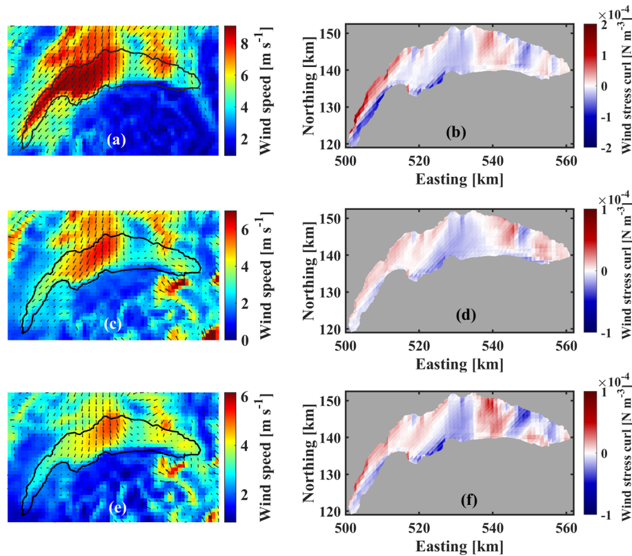
Figure 7. (a, c, e) Averaged wind speed and direction extracted from COSMO data for Bise events. (b, d, f) The computed wind stress curl for the corresponding Bise events. Panels (a) and (b) from 17 to 20 September 2019, (c) and (d) from 21 to 23 October 2019, (e) and (f) from 18 to 23 November 2019. Colour bars indicate the range of parameters.
