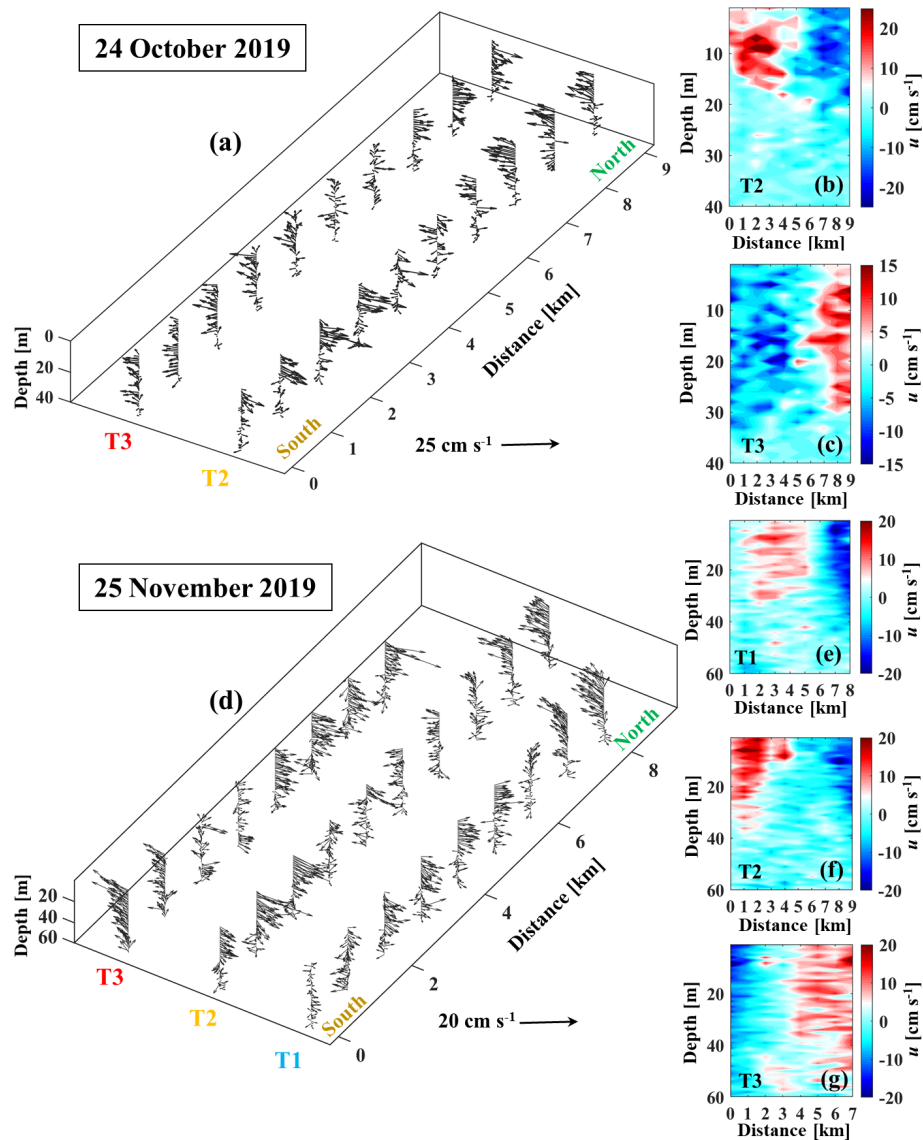
Figure 9. Field campaigns of October and November 2019 carried out along selected transects (T): (a) current velocity vector fields (arrows) of gyres AG (T3) and CG1 (T2) and (b, c) contour plots of the horizontal velocity, u , for 24 October 2019. (d) Current velocity vector field of gyres AG (T3), CG1 (T2), and CG2 (T1) and (e–g) contour plots of the horizontal velocity, u , for November 2019. The origin of the x axis is in the south. The colour bars indicate horizontal velocity in centimetres per second. Positive velocities are pointing eastward for transects T1, T2, and T3. For transect locations, see Fig. 1b.
