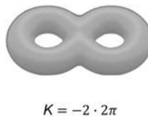
Figure 3. a. Examples of surfaces with positive (left), zero and negative (right) total Gaussian curvatures. b. Illustrations of closed surfaces and their respective total Gaussian curvature.
