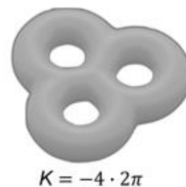
Figure 3. a. Examples of surfaces with positive (left), zero and negative (right) total Gaussian curvatures. b. Illustrations of closed surfaces and their respective total Gaussian curvature.
