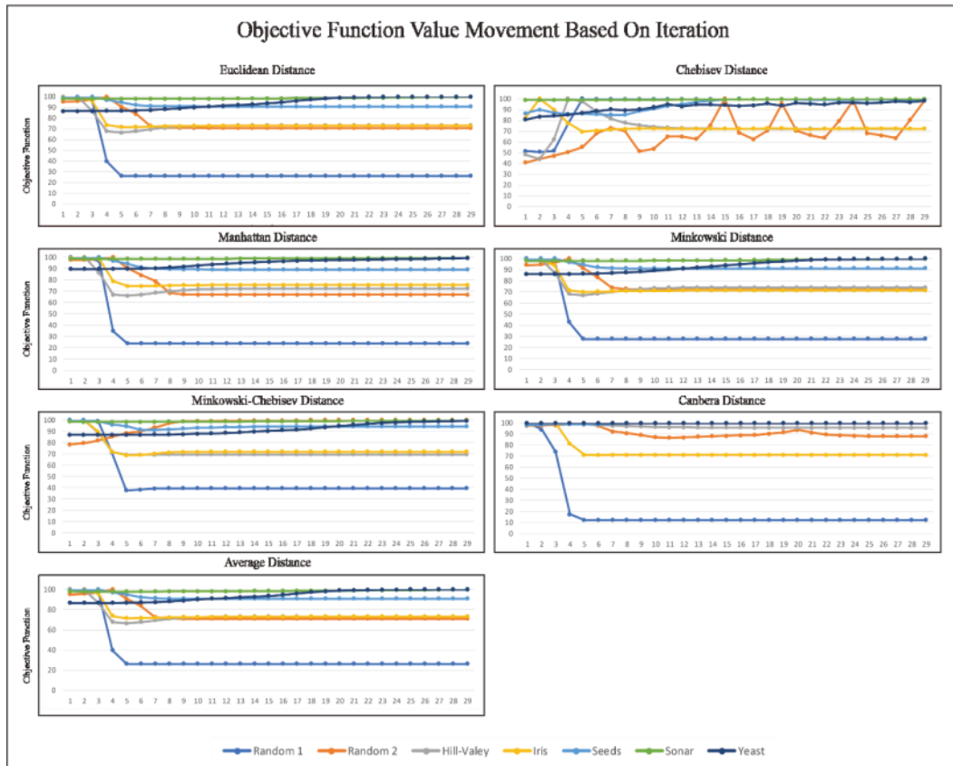
FIGURE 5. Objective Function Value Movement Based on Iteration
