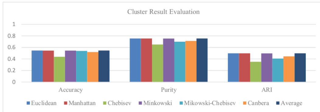
FIGURE 3. Cluster Result Evaluation
