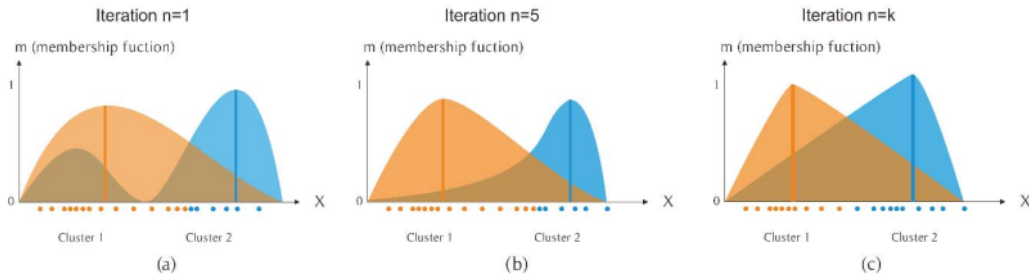
FIGURE 1. Membership Function Update During Iteration Process
