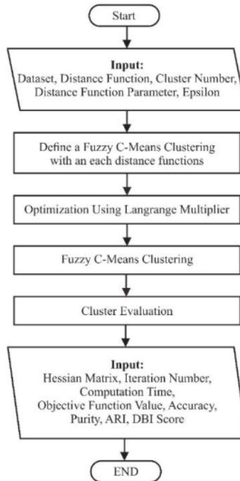
FIGURE 2. Research Flowchart
