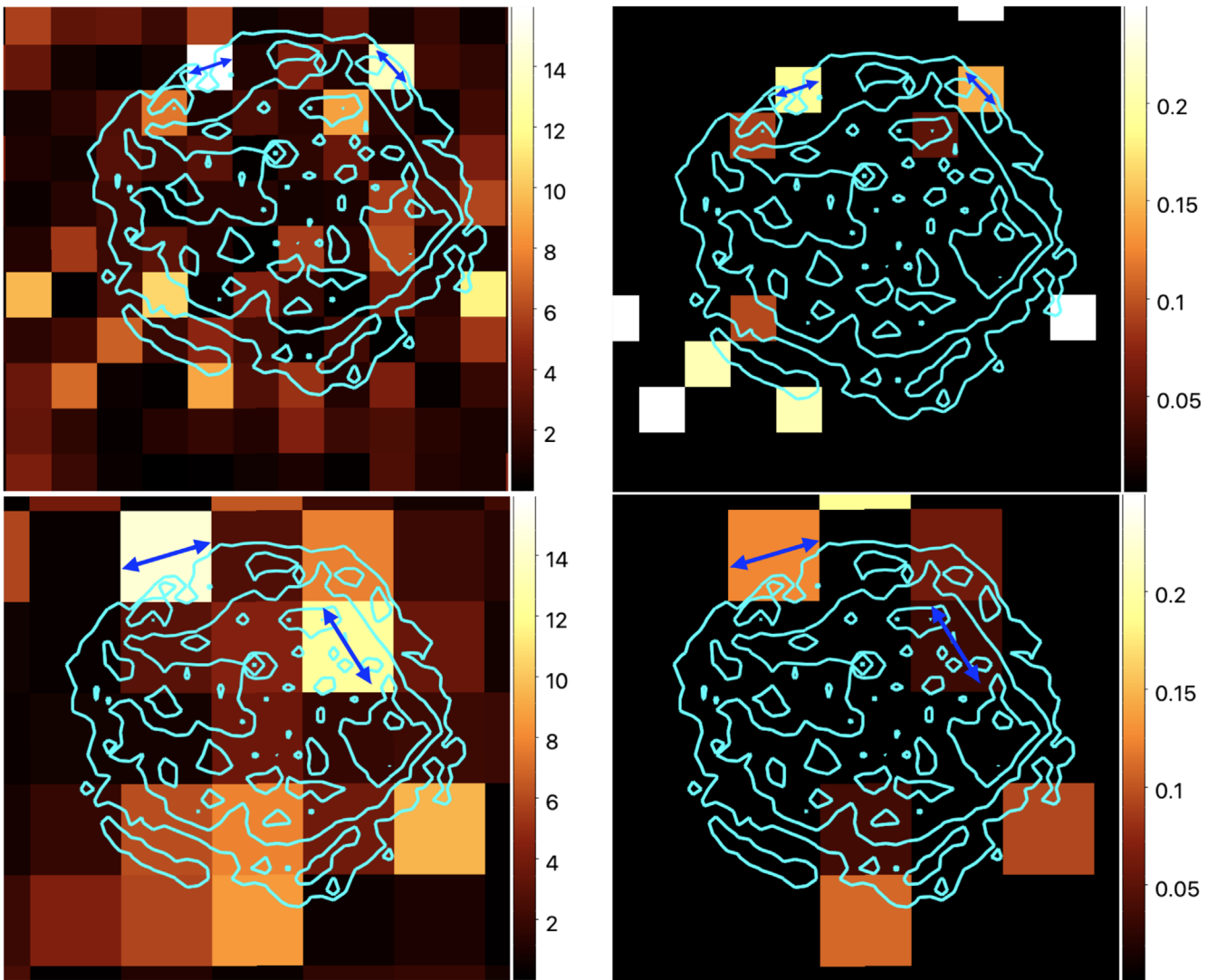
Figure 3. Left: maps of \chi^2 (or S_{ij} , see Appendix A) values for the polarization signal for the 3–6 keV band. Right: the corresponding polarization degree maps. Only pixels with pretrial confidence levels above 2\sigma ( \chi^2 > 6.28 ) are shown. For pixels with \chi^2 > 11.8 (corresponding to 3\sigma confidence level) the polarization angles are indicated with blue arrows. The errors on these angles are \sim 8^\circ . Top row: maps with pixel sizes binned to 42'' . Peaks in the \chi^2 map are \chi^2 = 15.9, 13.6 corresponding to polarization degrees of 19% and 14.5%. Bottom row: same plot, but with a larger pixel size of 84'' . Peaks in the \chi^2 map are \chi^2 = 14.4, 12.3 corresponding to polarization degrees of 12.4% and 3.4%.
