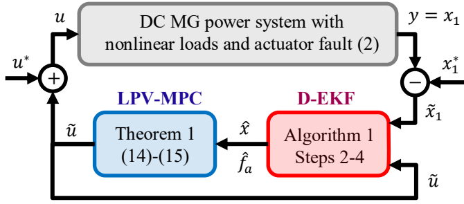
Fig. 6. Implementation of the proposed estimation method.
