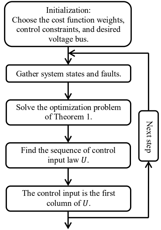
Fig. 4. LPV-MPC implementation.
