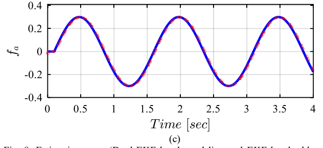
Fig. 8. Estimation error (Dual-EKF by the red line and EKF by the blue line): (a) voltage estimation, (b) current estimation, (c) actuator fault estimation.
