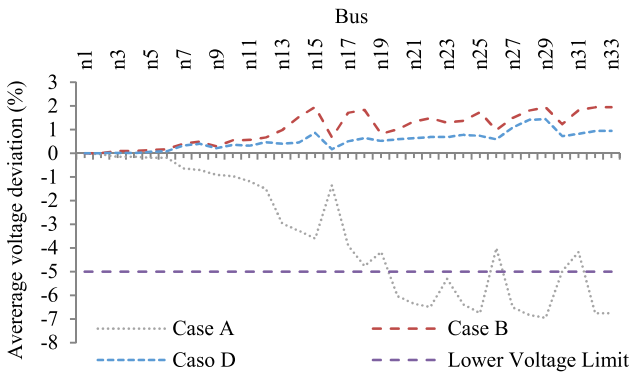
Fig. 10. Average voltage deviation profile of Cases A, C, and D in the Lagoa test system.
