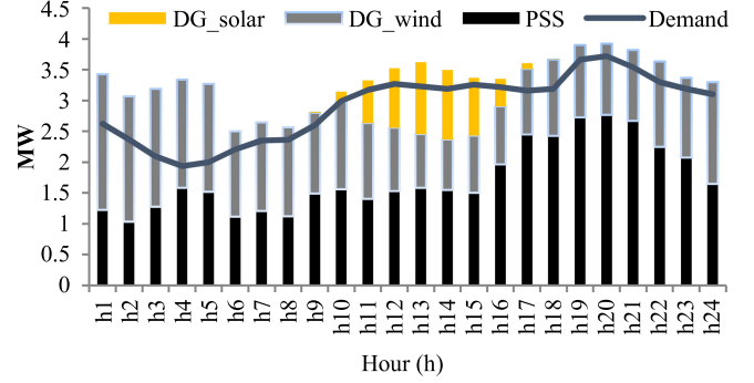
Fig. 6. Case C energy mix for Lagoa test system.
