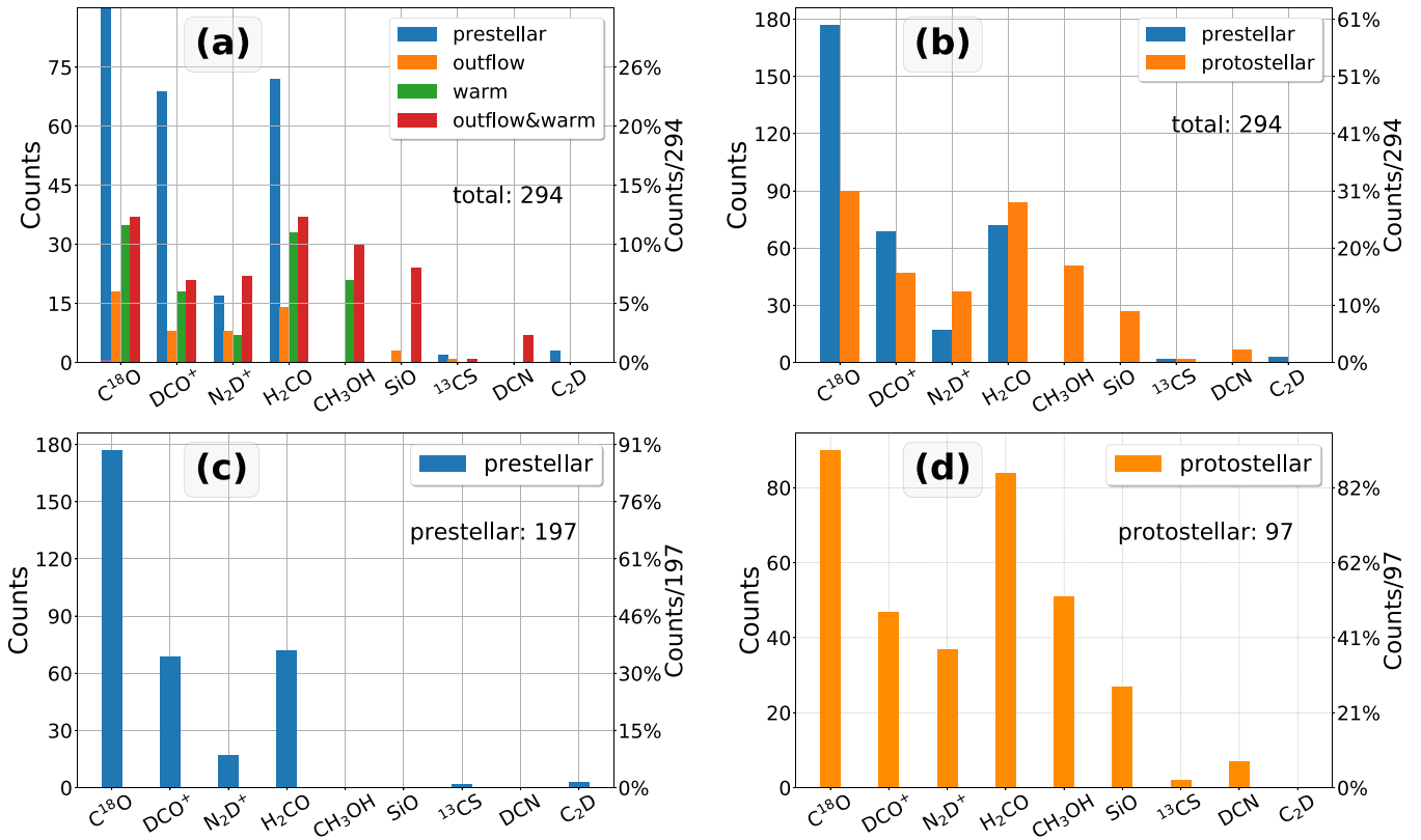
Figure 2. Histograms of the number and detection rate distributions of detected lines for: each evolutionary category of cores (a); prestellar vs. protostellar cores (b); prestellar cores only (c); and protostellar cores only (d).
