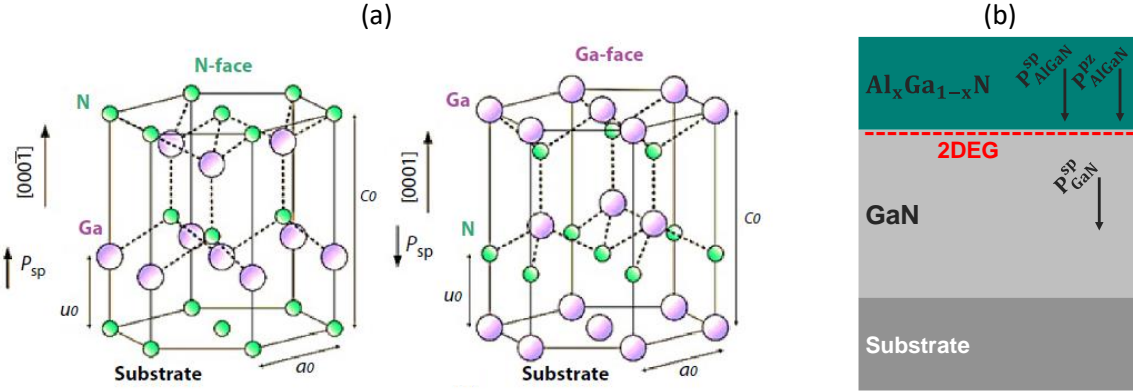
Figure 2: a) illustration of the lattice structure of GaN with Ga-face and N-face polarity – after [26]. b) illustration of ( AlGaN/Ga -face GaN) heterojunction with the polarization-induced 2DEG in the GaN layer.
