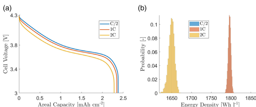
Figure 8. Results of case study with the battery cell model: a) discharge curves and b) uncertainty analyses at different C-rates.
