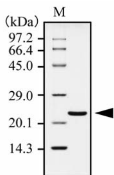
Figure 1. Sodium dodecyl sulfate-polyacrylamide gel electrophoresis image of coomassie brilliant blue R-250-stained purified recombinant sortase A with 59 amino acids deleted from the N-terminus and replaced with a His-tag (1 \mu g/lane).
