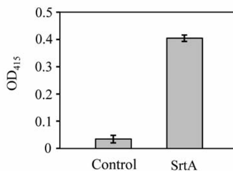
Figure 4. Surface modification of liposomes by recombinant sortase A with 59 amino acids deleted from the N-terminus and replaced with a His-tag ( His-ΔN 59 SrtA ) under the preferred condition. Biotinylated LPETGG peptide ( Bio-LPETGG ) was transferred onto the surface of G 5 liposomes by His-ΔN 59 SrtA at pH 6.5. The transferred Bio-LPETGG was detected by an enzyme-linked streptavidin assay using 2,2'-azino-bis(3-ethylbenzothiazoline-6-sulfonic acid) as a chromogenic substrate after incubation with horseradish peroxidase-labeled streptavidin.
