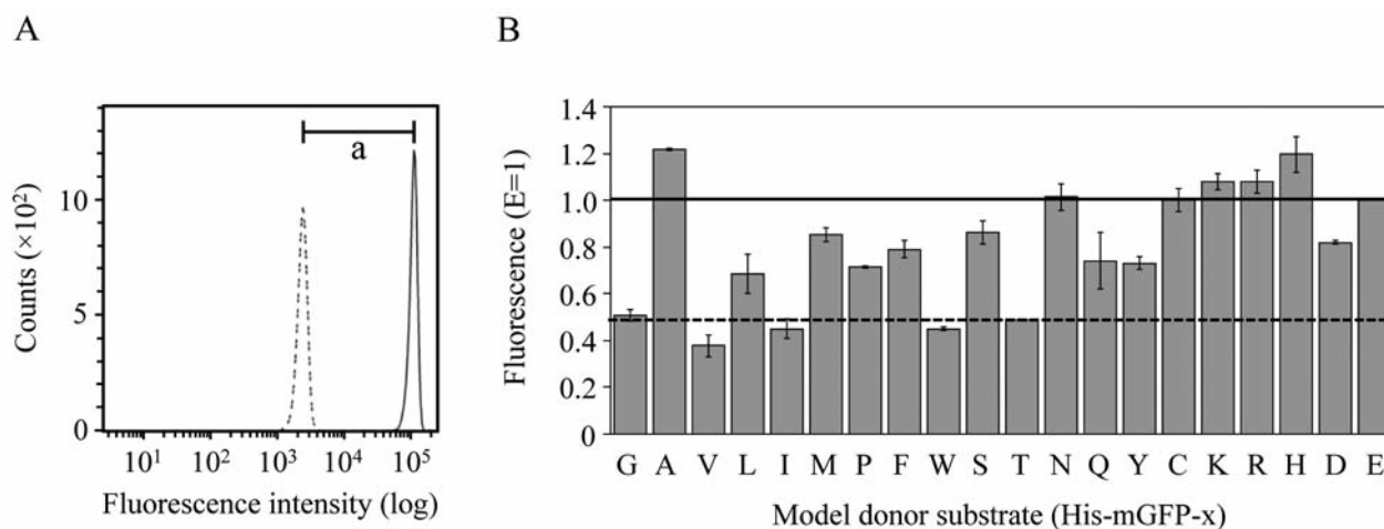
Figure 3. Evaluation of the preferred transpeptidase activity of recombinant sortase A with 59 amino acids deleted from the N-terminus and replaced with a His-tag ( His-ΔN 59 SrtA ). A: The histograms of the His-tagged mutant green fluorescent protein with a LPETGG-type sorting signal ( His-mGFP-E ) transferred onto G 5 beads and their background control were analyzed using a FACSVerse cell analyzer. A representative result for His-mGFP-E transpeptidation is shown. The difference between the median values of the histogram for the reaction mixture with and without His-ΔN 59 SrtA (shown as 'a') was calculated and used as the index of the transpeptidase reaction. B: The transpeptidase reaction of His-ΔN 59 SrtA with His-mGFP-x under preferred conditions. The result is shown as the ratio of the transferred His-mGFP-x to control His-mGFP-E .
