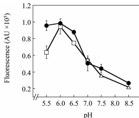
Figure 2. Transpeptidase reaction of recombinant sortase A with 59 amino acids deleted from the N-terminus and replaced with a His-tag (His- \Delta N 59 SrtA) under weakly acidic conditions. The transpeptidase reaction of His- \Delta N 59 SrtA was observed by measuring mutant green fluorescent protein (mGFP) fluorescence using a FACSVerse cell analyzer. The results show the transfer of His-tagged mGFP with a LPETGG-type sorting signal (His-mGFP-E) to G 5 beads under different pH. Closed circle, IBS (10 mM imidazole, 150 mM NaCl, pH 5.5-8.5); open square, MES-buffered saline (10 mM MES, 150 mM NaCl, pH 5.5-7.0); open triangle, HEPES-buffered saline (10 mM HEPES, 150 mM NaCl, pH 7.0, 7.5, and 8.5). Data are expressed as the mean \pm difference.
