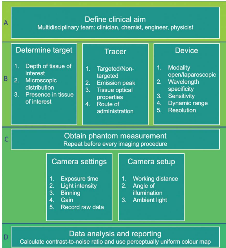
Figure 1: Checklist for performing in vivo fluorescence imaging studies. A step-by-step approach to ensure a standardized and reproducible FI clinical trial, including trial design, imaging acquisition, data analysis and reporting results. First, the clinician involved should define a clear and specific clinical aim in close cooperation with a chemist, engineer and physicist. The team then defines a biological target with the microscopic distribution and required penetration depth in mind. The tracer must match the target and should be selected based on the targeted/non-targeted approach, the tracers' emission peak, the tissue optical properties and the administration route. Simultaneously, the device emission and excitation filters must match the tracers' wavelength. Also, the form factor should be determined along with the desired resolution, sensitivity to light and dynamic range. Prior to every imaging procedure, phantom measurements should be obtained to evaluate performance characteristics over time. The user should set the camera settings such as exposure time, binning, gain, emission light intensity, and the data should be recorded without any pre-processing. Moreover, the camera setup should be identical in every procedure, with respect to the working distance, angle of illumination and ambient light levels, to compare results across patients. After data analysis, the performance of fluorescent tracer and imaging device combination should be reviewed based on the contrast-to-noise ratio. Images should be processed using perceptually uniform colour maps.
