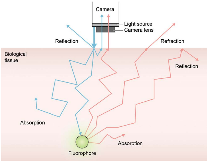
Figure 2: Basic principles of fluorescence and tissue optical properties. Fluorescent contrast generation starts with illuminating tissue at the appropriate wavelength for excitation of the fluorophore (i.e., endogenous or exogenous contrast). The fluorophore is excited from a ground state to an excited state by short-lived light absorption. Immediately after excitation, the fluorophore relaxes to a lower energy state and emits light of lower energy and longer wavelength than the excitation light. The emitted light propagates out of the tissue and is detected by the fluorescence detector that converts the recorded light into an image demonstrating the number of photons detected. Light propagation and imaging depth are limited by the tissue optical properties. Absorption causes light energy to be transferred to the tissue, decreasing the light intensity. Scattering is a process of short-lived absorption of a photon (typically) without energy loss, but with a change of initial direction. Also, scattering decreases the ability to distinguish details. If there is no correction for tissue optical properties, the signal registered is rather qualitative than quantitative.
