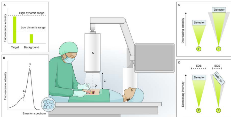
Figure 3: Potential pitfalls in fluorescence imaging studies. A. The contrast-to-noise ratio is strongly dependent on the dynamic range of the fluorescence imaging camera system concerning the fluorescent tracer. When imaging tissue using a fluorescent tracer with a high quantum yield, the system with the high dynamic range would result in a higher contrast-to-noise ratio compared to the low dynamic range system. B. The fluorescence intensity detected by the fluorescence imaging camera system is dependent on the match between the systems' optical filter and the emission peak of the fluorescent tracer used. A mismatch between the emission peak and optical filter will result in suboptimal fluorescence intensity detected (wavelength A) compared to the most optimal (wavelength B). C. The fluorescence intensity exponentially decreases with increased working distance due to the diverging nature of light. D. When the detector is not placed perpendicular to the tissue of interest, the effective detection surface (EDS) that can detect emitted photons is smaller. As such, fluorescence intensity is falsely reduced, possibly leading to erroneous conclusions.
