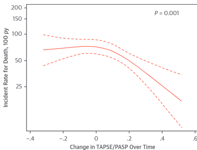
FIGURE 4 Continuous Association Between Change in TAPSE/PASP and All-Cause Death
