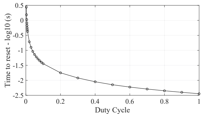
Fig. 11: Reset time of TCAMM CogniGron .
