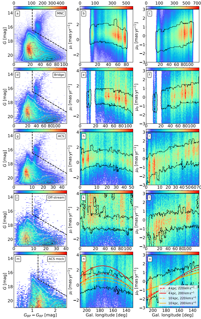
Fig. 5. CMD ( left ) and proper motion trends with Galactic longitude in \mu_l ( middle ) and \mu_b ( right ) of each structure. The CMDs contain the histogram of the stars within the highest intensity proper motion peaks (peak stars) with grey contours on top that represent the CMDs of all the stars in the region. The dashed black lines represent our selection of giant stars. The proper motion maps contain all the stars in the region, and the black line is the zero-contour of the peak stars, that is, the stars that fall within the highest intensity proper motion peak of their HEALpix. First row: MNC. Second row: bridge between MNC and the ACS. Third row: ACS. Fourth row: above the ACS. Fifth row: same region as the ACS but for the mock particles, selecting the stars for the CMD according to the contours of panels h and i . In the bottom panel we also include the proper motions expected from a structure 30^\circ above the plane at a given distance – 4 (red) or 10 (orange) kpc – rotating at a given velocity – 200 (solid) or 220 (dashed) \text{km s}^{-1} – but with no radial or vertical velocity.
