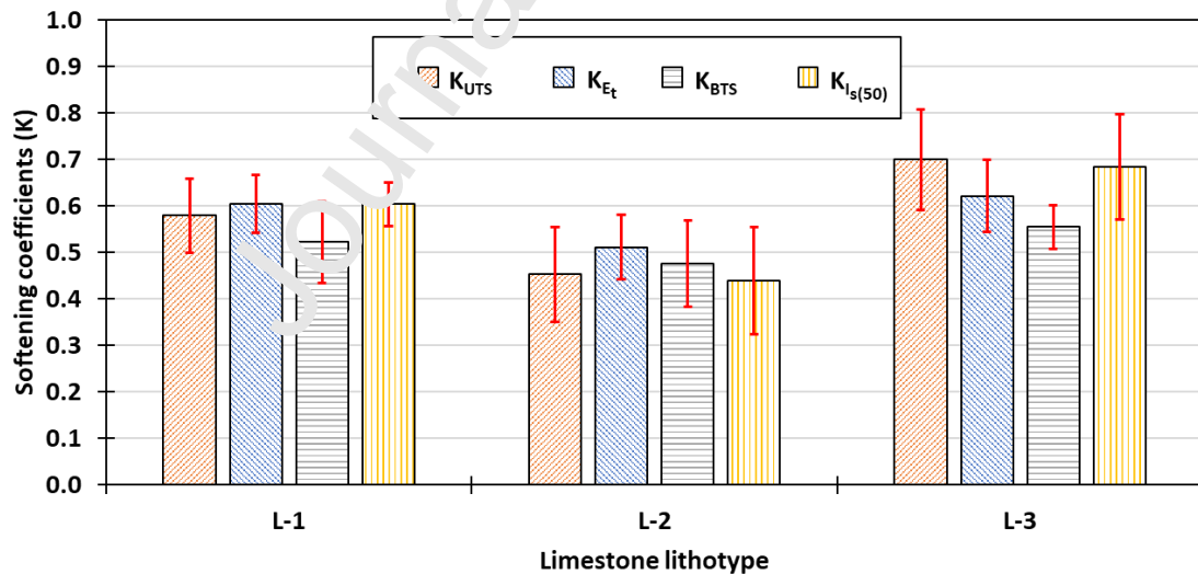
Figure 9. Softening coefficients obtained in the three tested limestone lithotypes. The error bars represent the standard deviation.
