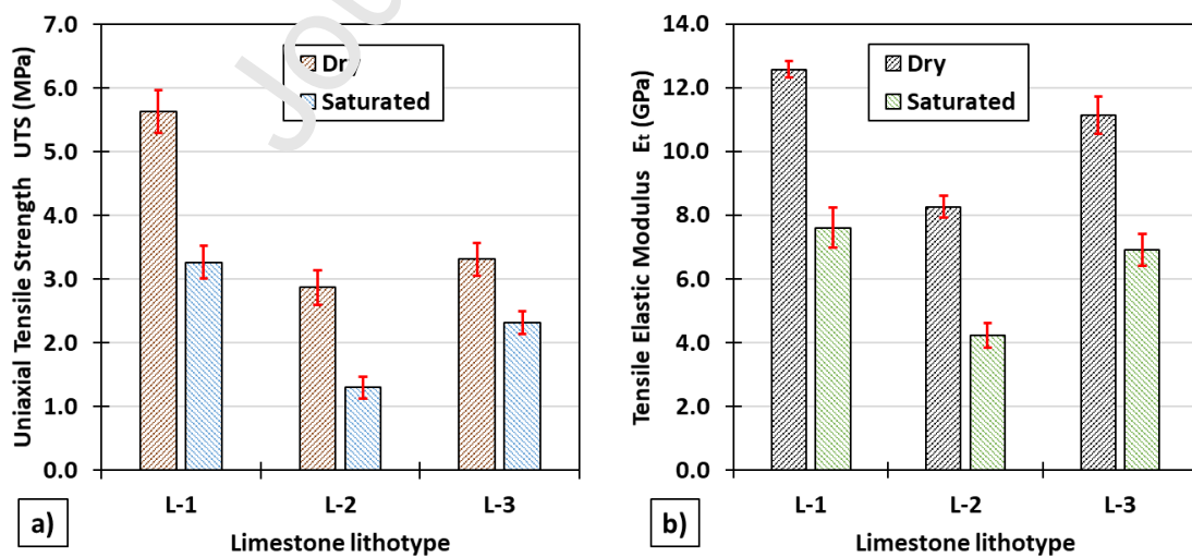
Figure 6. Comparison of the Uniaxial Tensile Strength (UTS) (a) and the Tensile Elastic Modulus ( E_t ) (b) values found in dry and water-saturated specimens of the three limestone lithotypes. The error bars represent the standard deviation.
