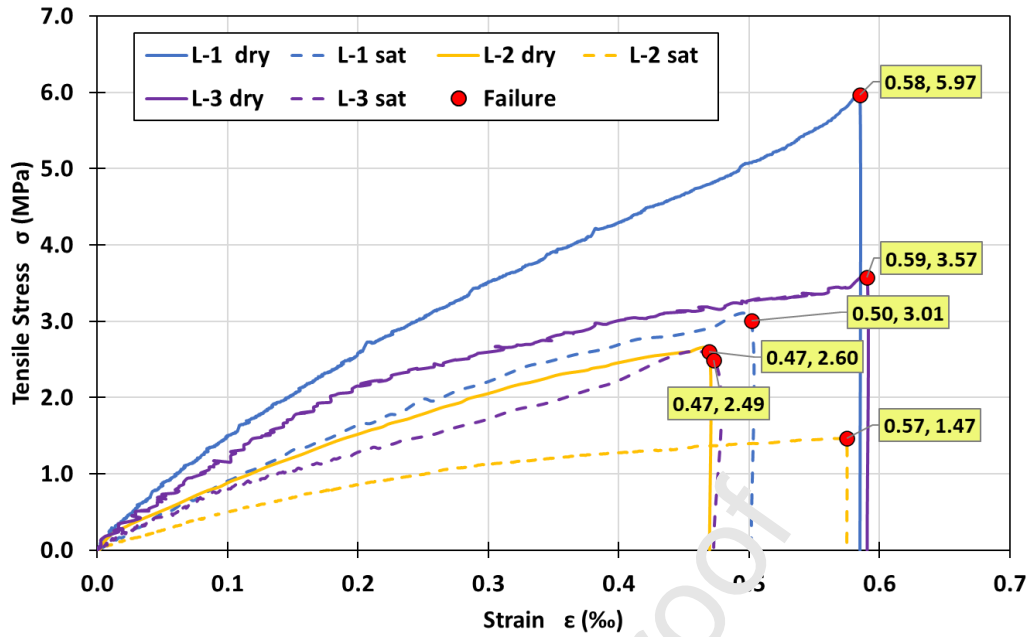
Figure 5. Representative examples of stress-strain curves obtained in uniaxial tensile direct-pull tests for dry and water-saturated specimens of the three limestone lithotypes.
