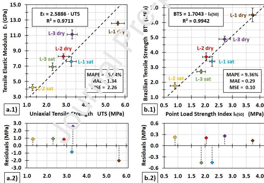
Figure 12. Relationships correlating Tensile Elastic Modulus ( E_t ) with Uniaxial Tensile Strength (UTS) (a.1) as well as Brazilian Tensile Strength (BTS) with Point Load Strength Index ( I_{s(50)} ) (b.1) found in tested limestones and their corresponding residual plots (a.2 and b.2, respectively). The error bars represent the standard deviation.
