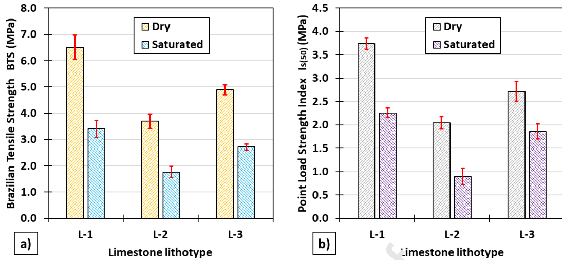
Figure 8. Comparison of the Brazilian Tensile Strength (BTS) (a) and the Point Load Strength Index ( I_{s(50)} ) (b) values found in dry and water-saturated specimens of the three limestone lithotypes. The error bars represent the standard deviation.
