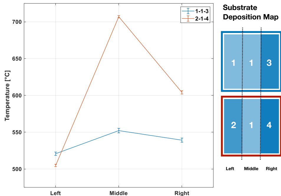
Figure 7. Comparison of two substrates with tailored catalyst distribution. T_{substrate} is compared within three regions coated with 1, 2, 3, and 4 sides coated. The substrate map on the right provides the number of coats received by the two tailored substrates, i.e., 113 and 214. A single thermocouple was placed in the center of each region at a distance of 6.5 mm from each other with the center thermocouple directly in the middle of the substrate. Air flow rate of 6000 mL/min was maintained.
