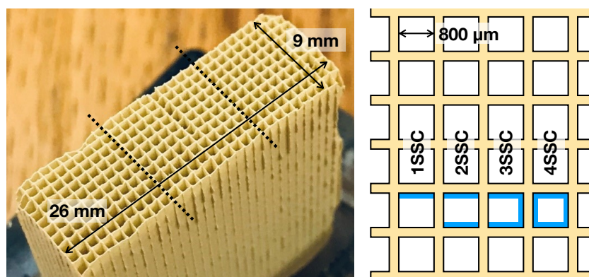
Figure 1. An image of cleaned cordierite cartridge prior to catalyst coating. The illustration shows four deposition procedures used for incremental addition of loading and the tailored distribution study. For instance, 2SSC samples had two sides with single catalyst coating depicted in blue.
