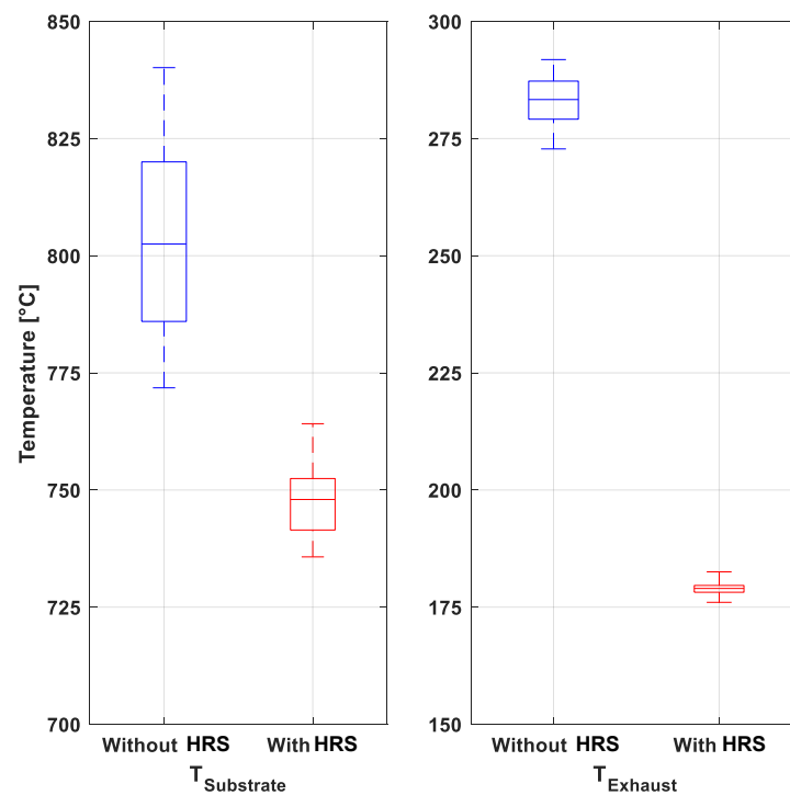
Figure 4. Comparison of the reactor with and without the Heat Recirculation System (HRS) composed of top and bottom units. The implemented HRS decreased the exhaust temperature by \sim 100 °C averaged over the two units. Air flow was 6000 mL/min through 2SSC substrates.
