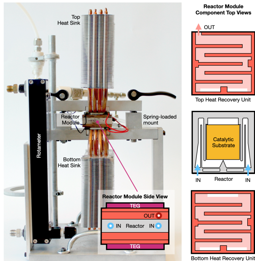
Figure 2. The modified facility is 15 inches in height with a 8 in x 8 in baseplate. The facility includes: a rotameter, bubbler, two heat exchangers, and a reactor assembly that integrates spring-loaded clamps to uniformly distribute pressure across the reactor. Within the layered reactor shown as an inset, the methanol-air mixture enters through the two inlet ports (depicted with blue arrows), travels through the catalytic substrate (illustrated in orange) where combustion occurs, down and across the Bottom Heat Recovery Unit, routed up through two slots in the reactor wall and across the Top Heat Recovery Unit to an outlet port (depicted with an orange arrow).
