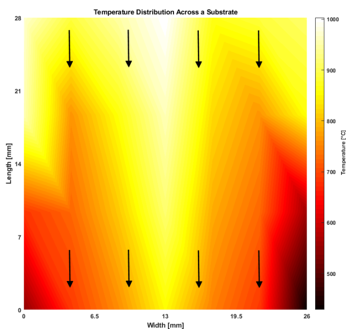
Figure 6. Thermal map of the substrate temperatures, T_{substrate} , across the middle of the catalytic substrate. Black arrows indicate the direction of flow. The experiment was conducted with 6000 mL/min air flow through a 2SSC substrate.
