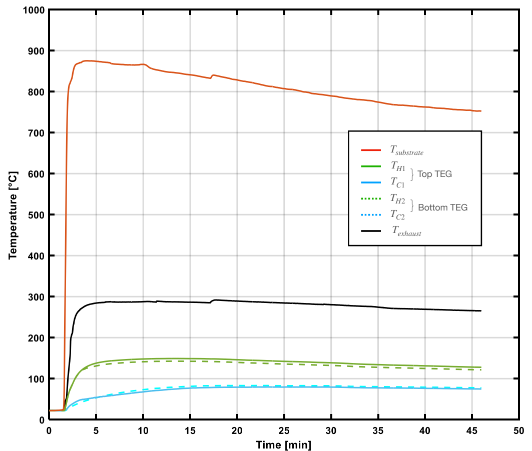
Figure 3. Temperature histories of microcombustion reactor facility without the thermal management modifications. The experiment was run at 6000 mL/min air flow rate with a 2SSC substrate. T_{substrate} represents the temperature at the center of the substrate. T_H and T_C represent the hot and cold side temperatures, respectively, of the top and bottom TEG modules. T_{exhaust} is the reactor exhaust temperature.
