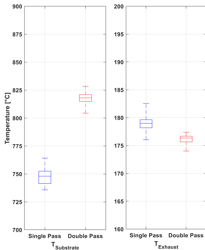
Figure 5. A comparison of mean temperatures T_{\text{substrate}} and T_{\text{exhaust}} for the single pass and double pass inlets at 6000 mL/min air flow rate with 2SSC substrates.
