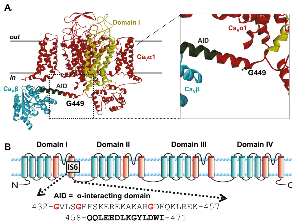
Figure 1. The \text{Ca}_V1.2 variant is located in the intracellular linker before the binding site for the \text{Ca}_V\beta subunit. The LQTS-related \text{Ca}_V\alpha1C mutation G449 is located before the \alpha -interacting domain (AID). A , the cryo-EM 3D structure of the rabbit \text{Ca}_V1.1 oligomeric complex at 3.6 Å for \text{Ca}_V\alpha1S and at 3.9 Å for \text{Ca}_V\beta (Protein Data Bank code: 5GJV). \text{Ca}_V\alpha1C and \text{Ca}_V\alpha1S share 81% homology in their primary protein sequence. L-type calcium channels share similar structure, being composed of the pore-forming subunit \text{Ca}_V\alpha1 in red and \text{Ca}_V\beta in blue and an intracellular subunit bound to \text{Ca}_V\alpha1 through the intracellular helix linking domains I and II of \text{Ca}_V\alpha1 (shown in dark green). The first transmembrane domain of \text{Ca}_V\alpha1 (DI) is shown in yellow. The human LQTS-related \text{Ca}_V\alpha1C G419R variant is similar to the rabbit \text{Ca}_V\alpha1C G449R and is equivalent to Gly358 in \text{Ca}_V\alpha1S . Image was produced by Discovery Studio 2020 (BIOVIA Pipeline Pilot 2020). B , cartoon of the corresponding secondary structure for the \text{Ca}_V\alpha1C pore-forming subunit of the L-type \text{Ca}_V1.2 channel showing the four homologous domains (domains I to IV) with the N and C termini located into the cytoplasm. The \text{Ca}_V\beta subunit-binding site on the \text{Ca}_V\alpha1C subunit is referred to the “ \alpha -interacting domain” or AID. The AID is located within 20 residues of the sixth transmembrane segment in domain I (IS6). The primary sequence for the AID motif is shown below the primary sequence for the short region extending from the end of S6 to the beginning of the AID. The relative position of three glycine variants reported in the Timothy syndrome (G402S, G406R, and G419R) is fully conserved across species and presented in red with the numbering in the rabbit clone used for this study. LQTS, long-QT syndrome.
