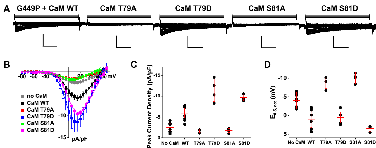
Figure 9. Ca_v1.2 G449P is modulated by CaM phosphorylation surrogates. A , whole-cell currents were recorded from HEK293T cells transiently transfected with Ca_v1.2 G449P coexpressed with Ca_v\beta2a and Ca_v\alpha2\delta1 and either CaM WT, with the phosphoresistant CaM (T79A or S81A), or with phosphomimetic CaM (T79D or S81D) as indicated. Exemplar traces are shown (from left to right) for Ca_v1.2 G449P + CaM WT, G449P + CaM T79A, G449P + CaM T79D, G449P + CaM S81A, and G449P + CaM S81D. The vertical scale bars are 10 pA/pF, and the horizontal scale bars are 100 ms throughout. B , the corresponding peak current densities are plotted as a function of applied voltage. C and D , the summarized distribution of the peak current densities and the midpoint of activation E_{0.5,act} . Peak whole-cell currents and E_{0.5,act} are reported individually as black circles. The mean data \pm SD are shown as red hyphens. Values of peak current densities and E_{0.5,act} are reported in Table 6. CaM, calmodulin; HEK293T, human embryonic kidney 293T cell line.
