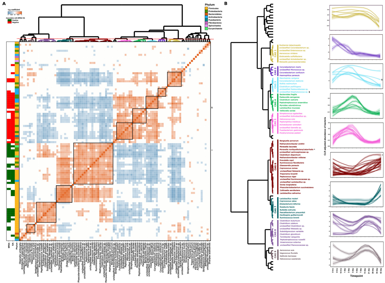
FIG 4 Longitudinal dynamics of bacterial species comprising coabundant groups (CAG) in 16S rRNA gene sequencing. (A) Heatmap plot of the r_m coefficient values between each pair of species-level taxa. CAGs were obtained based on clustering of r_m coefficient values by Spearman correlation and ward linkage hierarchical clustering. Cutting the dendrogram at a height of 1.0 allowed us to identify nine different CAGs. Taxa showing significant association with MRSA/ S. aureus nasal colonization as measured by the rmcorr package are displayed as sidebars ( r_m coefficient). A phylum-level grouping of each individual species is displayed as the leftmost side bar. (B) Longitudinal dynamics of each species based on their identified CAGs across the time points. Species comprising different CAGs have been identified and annotated on a dendrogram based on their CAG assignment. Each individual line chart displays within-CAG dynamics of bacterial species across the time points, and the colors of the lines are matched according to their CAG assignment. Each line represents a single species.
