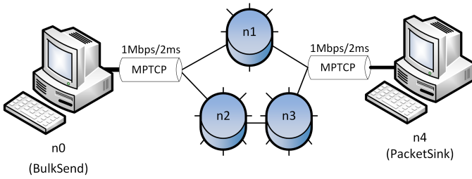
Figure 5: Testbed topology
