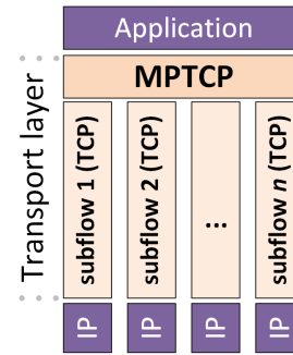
Figure 1: MPTCP stack
