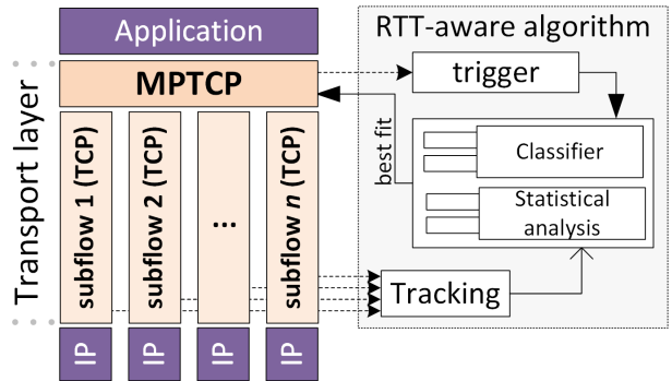
Figure 3: RTT-aware algorithm
