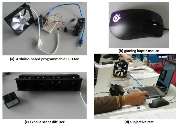
Fig. 2: Mulsemmedia Equipment and Test-bed
