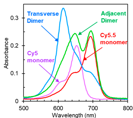
Figure 1. Steady-state absorption spectra of DNA-templated Cy5 and Cy5.5 monomers and heterodimers in 1× TAE buffer with 15 mM MgCl 2 added and measured at room temperature. “Adjacent” and “transverse” describe the relative position of the dyes in the Holliday junction as shown in Scheme 1.
