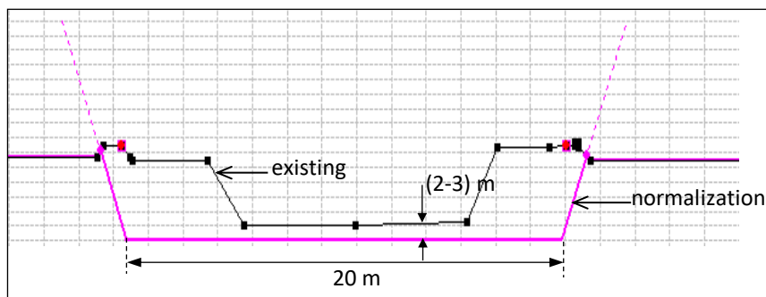
Figure 4. Normalization Planning of River Cross-Section
