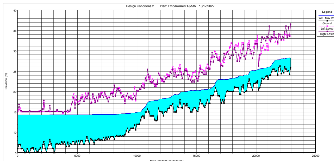
Figure 6. Water surface profile after normalization and embankment with Q_{25y}
