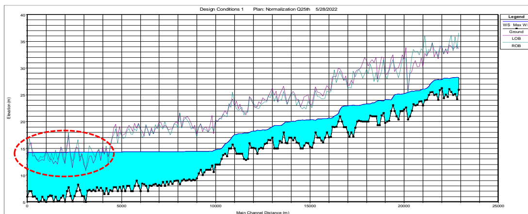
Figure 5. Water surface profile after Normalization
