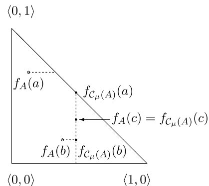
Figure 4 Operator C_\mu
