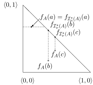
Figure 9 Operator \mathcal{I}_\nu^*
