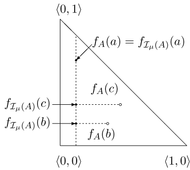
Figure 6 Operator \mathcal{I}_\mu
