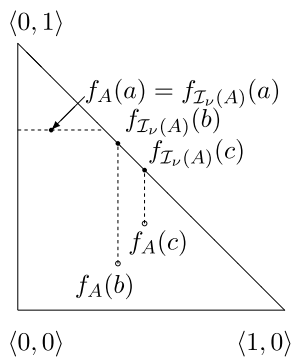
Figure 7 Operator \mathcal{I}_\nu
