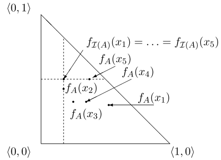
Figure 3 Operator I
