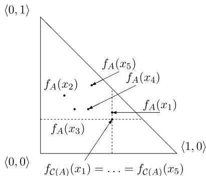
Figure 2 Operator C
