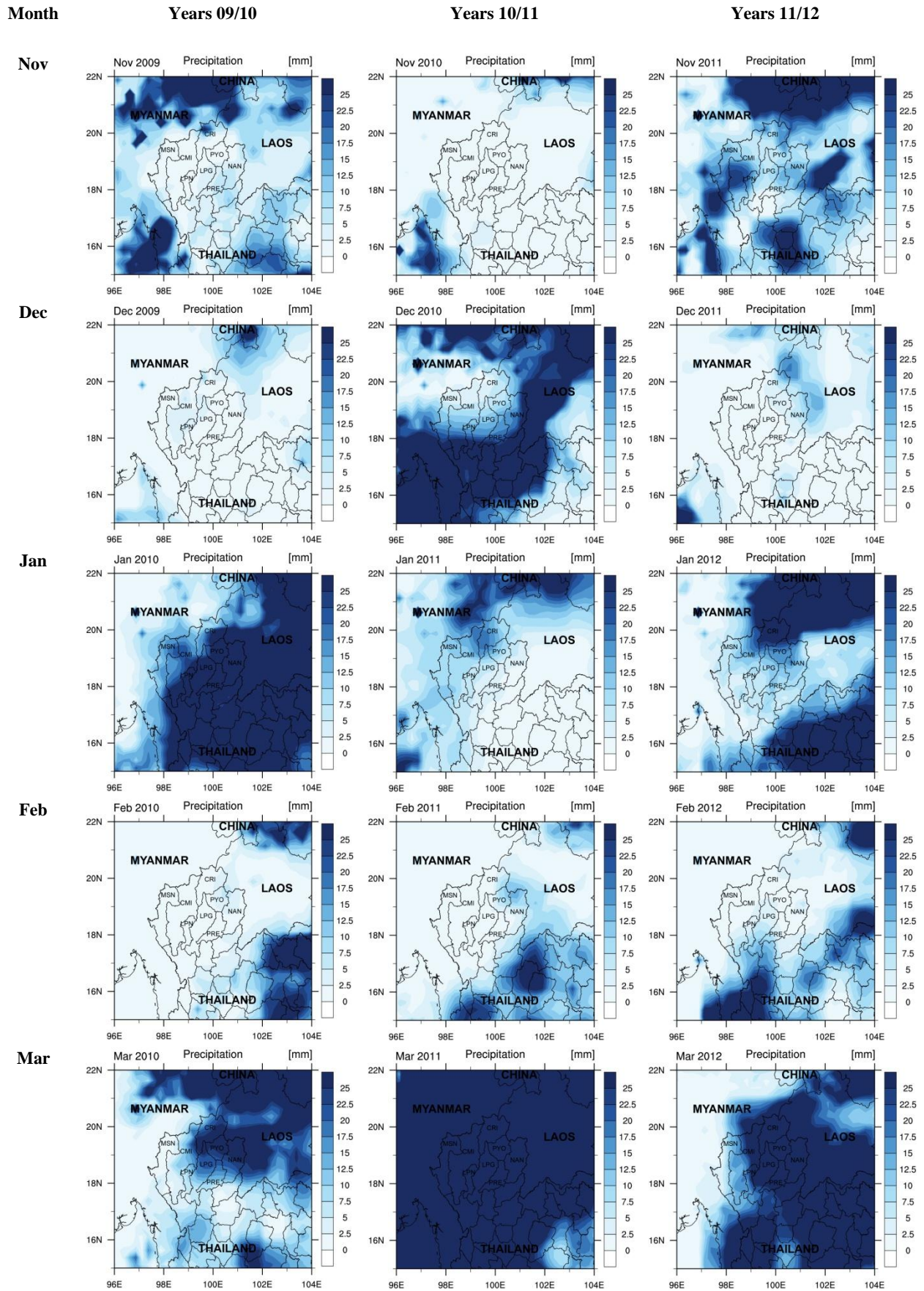
Figure 4 Monthly accumulated precipitation (TRMM data).
