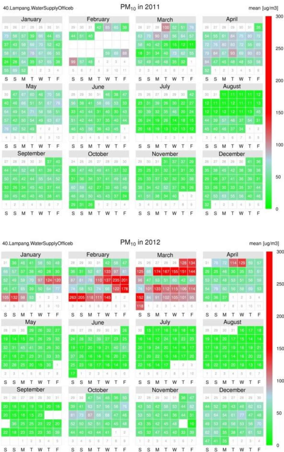
Figure 2 Calendars of PM 10 concentrations (24-hour average values) from 2009 to 2014 of the Lampang station (ID.40) (continued).
