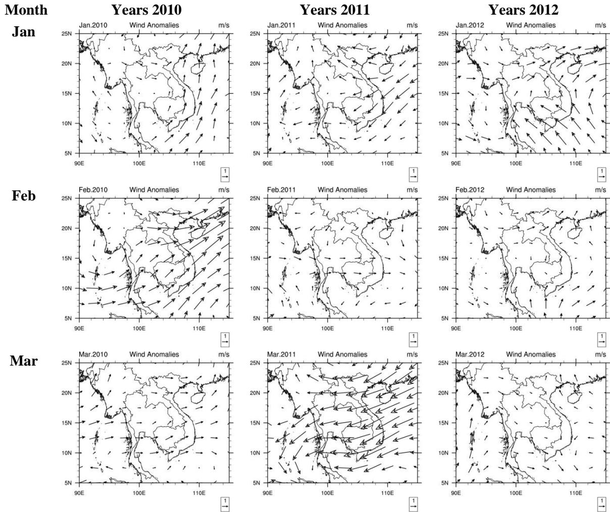
Figure 6 Wind anomalies at 850 hPa on January, February, and March in 2010, 2011, and 2012.
