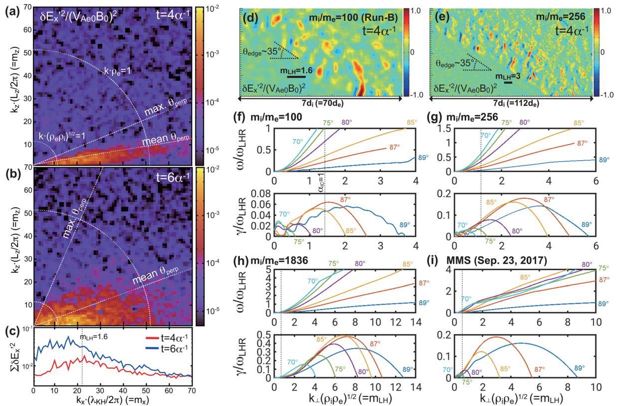
FIG. 7. (a)–(c) 2D power spectra ( k_x, k_z ) of E_x^2 and sum of the spectra in k_z at t = 4 and 6\alpha^{-1} around the center of the boundary ( y = 0 \pm 5d_i ) for run-B. The dotted lines in (a) and (b) indicate the angle of the perpendicular direction to the magnetic field in the x - z plane \theta_{\text{perp}} at the head of the high-density arm, the maximum and mean \theta_{\text{perp}} on the low-density side of the density gradient layer defined as the region with 0.2 < n_e/n_0 < 0.4 , and the wavelengths for k_{\perp}\rho_e = 1 and k_{\perp}(\rho_i\rho_e)^{1/2} = 1 . (d) The zoomed-in view of the E_x^2 contour in the region marked in Fig. 6(d). (e) The same as (d), but for an additional run with m_i/m_e = 256 . (f)–(i) Linear dispersion relations at the edge of the KH waves derived by Umeda and Nakamura (2018). Panels show wave modes with wave normal angles quasi-perpendicular to the ambient magnetic field ( \phi = 70^\circ - 89^\circ ) for parameters, obtained from the simulation near the compressed density gradient layer at t = 4\alpha^{-1} marked in Fig. 4(b) (f), similar to (f) but for m_i/m_e = 256 (g) and m_i/m_e = 1836 (h), and obtained from the MMS observations on September 23, 2017 Blasl et al. (unpublished).
