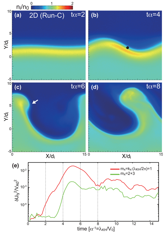
FIG. 4. (a)–(d) Time evolution of color contours in the x – y plane of n_i from t = 2 to 8\alpha^{-1} for the local 2D run (run-C), where \alpha^{-1} = \lambda_{\text{KH}}/V_0 is the time unit for the growth phase of the KHI (Nakamura et al. , 2013). (e) Time evolution of the 1D power spectra ( k_x ) of U_y modes ( m_x = 1 and m_x = 2 + 3 ) obtained by calculating the power of each mode at each y and then picking up the maximum value for each mode. Vertical dotted lines in (e) indicate the times shown in (a)–(d).
