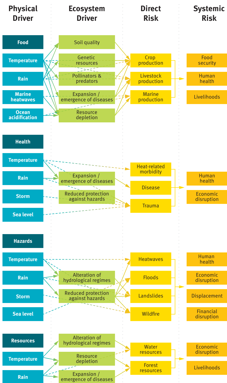
Figure 3: Overview of the effects of physical drivers and ecosystem changes on direct and systemic risks, for four areas
