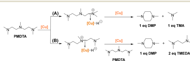
Scheme 3 Possible transalkylation paths for PMDTA transformation into DMP over Cu 3 [Cu] resulting in (A) TMA (1 eq. PMDTA) and (B) TMEDA (2 eq. PMDTA). Detailed catalytic cycles are provided in Scheme S2A and B † . Reaction conditions: 200 °C, 20 h, H 2 (50 bar), MeOH/PMDTA (molar) = 32, 100 mg of Cu 3 per 6 mmol of DETA. The catalyst was pre-reduced from 50 °C to 200 °C using a temperature ramp of 1 °C min -1 before the reaction.
