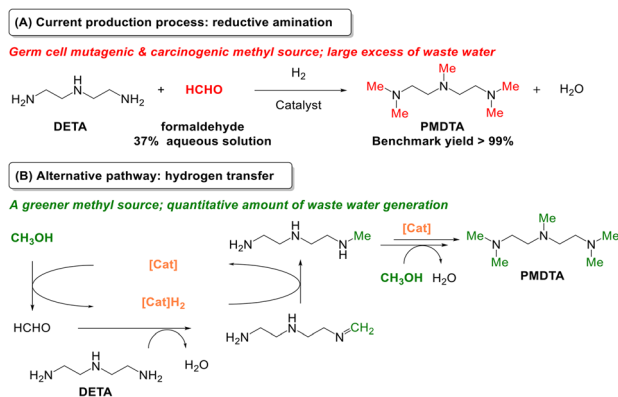
Scheme 1 (A) Current route for PMDTA synthesis from DETA and formaldehyde, and (B) alternative route for PMDTA synthesis from DETA and MeOH (CH 3 OH) under the hydrogen borrowing mechanism.
