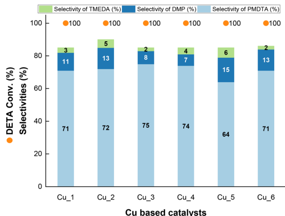
Fig. 2 Results of composite Cu catalyst screening for DETA methylation. Reaction conditions: 200 °C, 20 h, H 2 (50 bar), MeOH/DETA (molar) = 742, 140 mg of catalyst (64–109 mg Cu) per 1 mmol of DETA. The catalysts were pre-reduced from 50 °C to 200 °C using a temperature ramp of 1 °C min -1 before the reaction.
