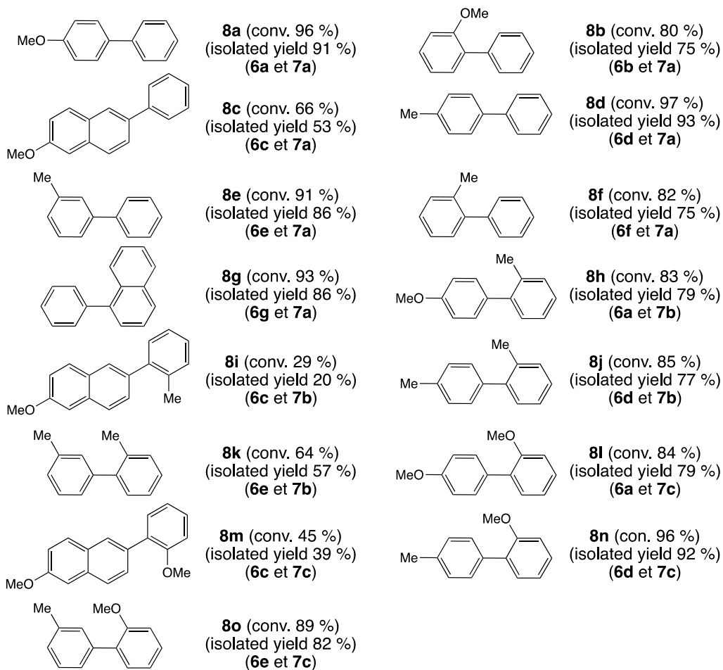
Figure 4. Palladium-catalyzed Suzuki–Miyaura cross-coupling: formation of biphenyls from aryl bromides and aryl boronic acids; reagents and conditions: [Pd(OAc) 2 ] (0.5 mol%), 1 (0.5 mol%), ArBr (0.5 mmol), Ar'B(OH) 2 (0.75 mmol), Cs 2 CO 3 (0.75 mmol), 1,4-dioxane (2 mL), decane (0.025 mL), 5 h, 100 °C. The conversions were determined by GC, the calibration being based on decane.
