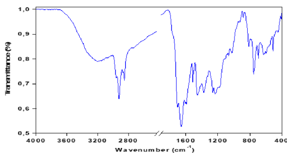
Figure 7. FTIR spectra of bio-oil produced by pyrolysis of red algal biomass ( T = 450\text{ °C} and \beta = 10\text{ °C}/\text{min} ).
