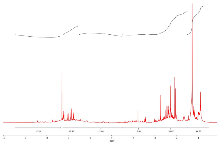
Figure 8. ^1\text{H-NMR} spectra of bio-oil produced by pyrolysis of red algal biomass ( T = 450\text{ }^\circ\text{C} and \beta = 10\text{ }^\circ\text{C}/\text{min} ).
