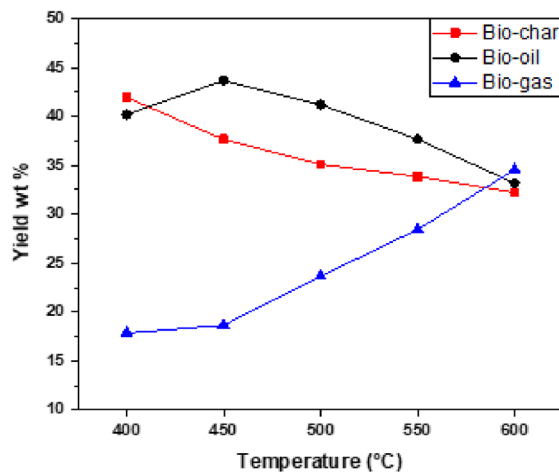
Figure 4. Effect of final pyrolysis temperature on product yields at a heating rate of 15\text{ °C/min} .
