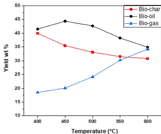
Figure 5. Effect of final pyrolysis temperature on product yields at a heating rate of 30\text{ °C/min} .
