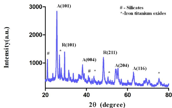
Figure 4. XRD analysis of the freshly coated composite.
