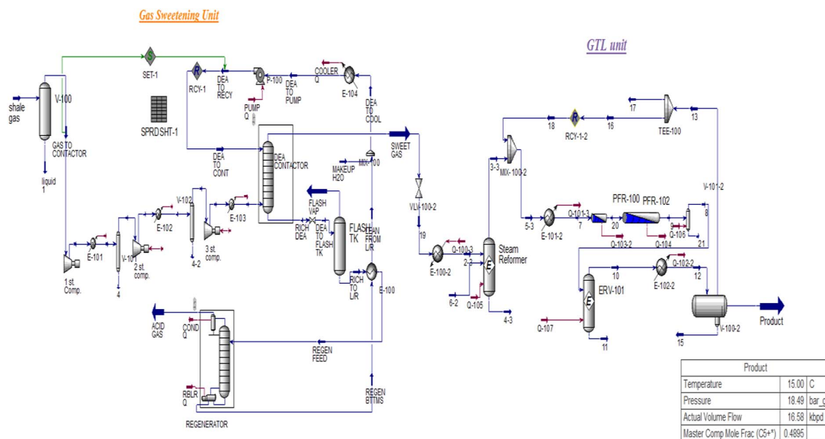
Figure 1. Process flow diagram of GTL unit.
