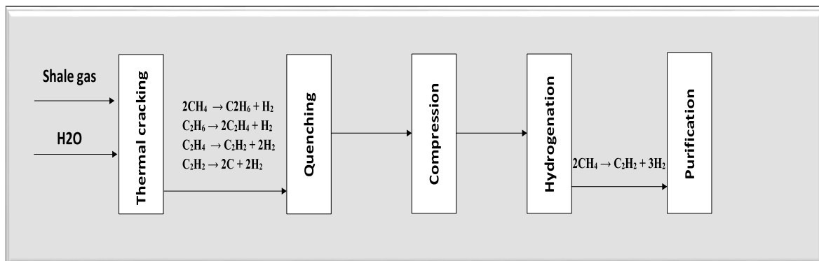
Figure 5. Schematic of the GTL process.
