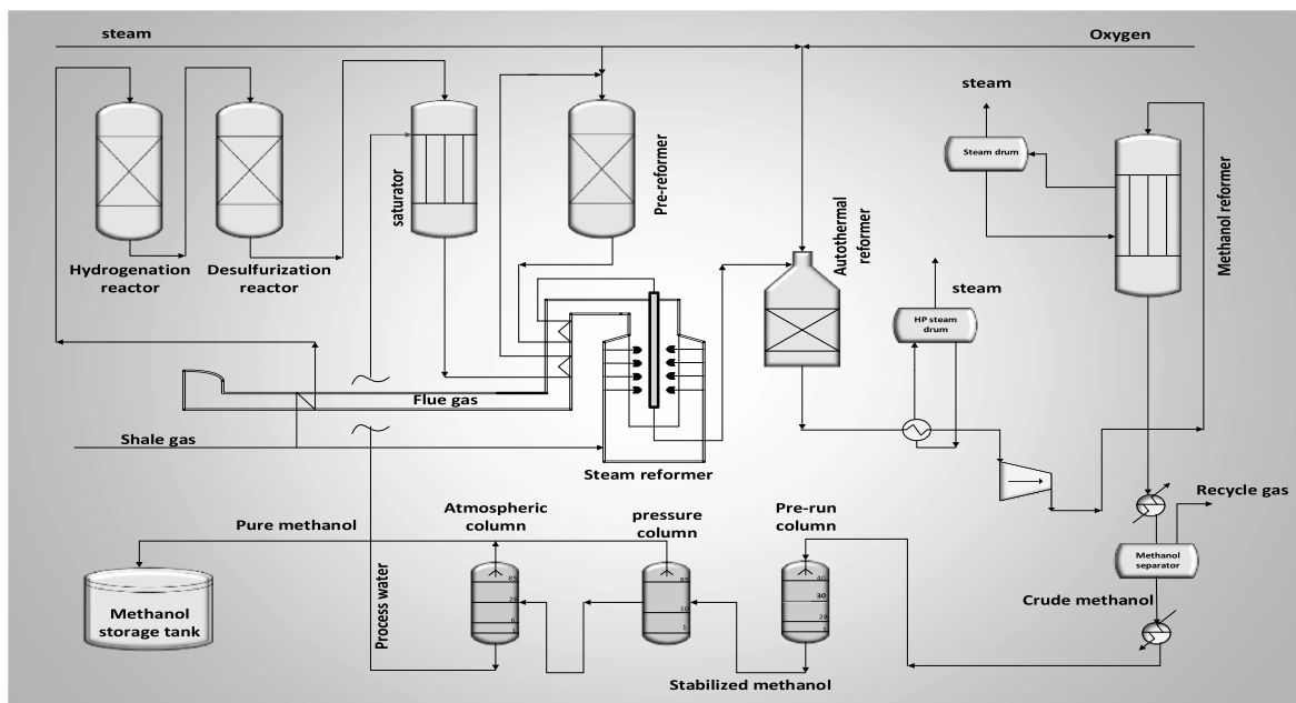
Figure 2. Block diagram of GTM unit.
