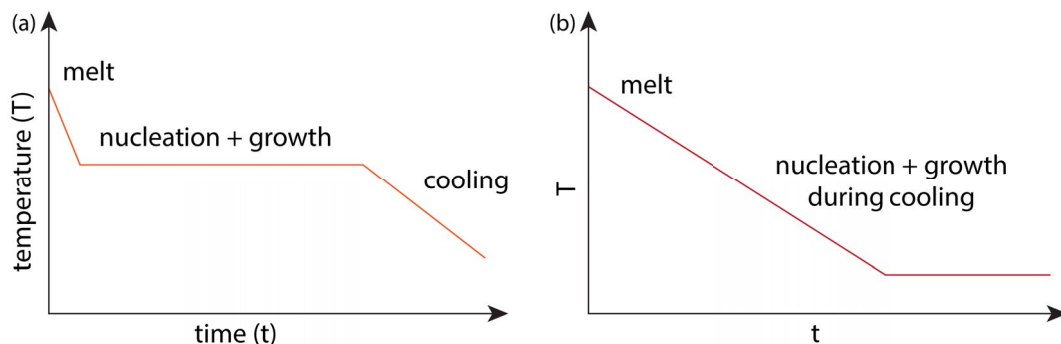
Figure 6. Schemes used for GCs produced from nuclear waste in order to avoid having to reheat quenched glass.
