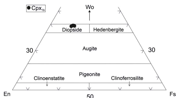
Figure 8. Clinopyroxene (Cpx 1b ) classification in the Wo–En–Fs diagram.
