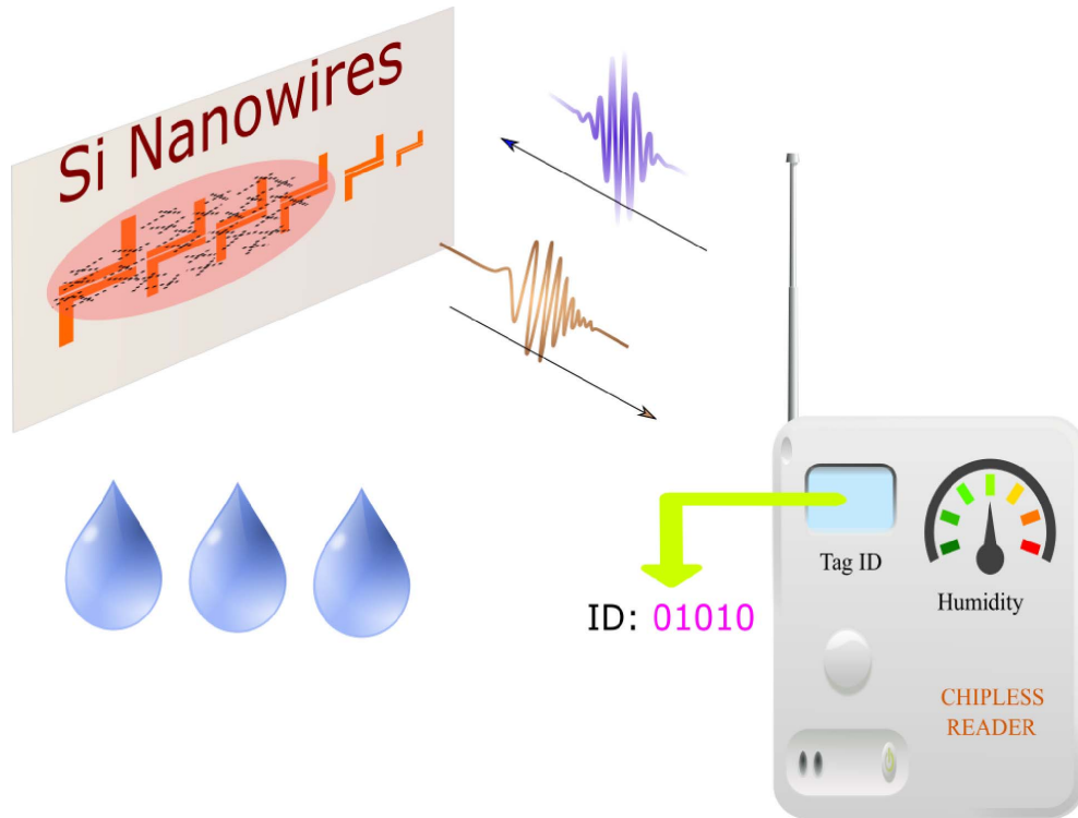
Figure 7. Illustration of the reading of a chipless tag with an identifier and a humidity sensor. Resonators are either used to encode the information or to read the relative humidity in the air. In this example, a humidity-sensitive material (silicon nanowires—SiNw) has been deposited on these resonators. Therefore, the resonance frequency associated with these specific resonators (with SiNw) will change according to the relative humidity level. The measurement of the 6 resonance frequencies allows the recovery of the tag’s ID and the humidity value in one go.
