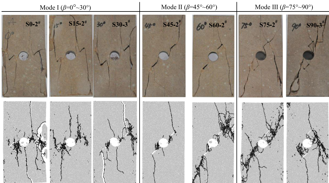
Figure 13. Comparison of ultimate failure modes between laboratory tests and numerical simulation.
