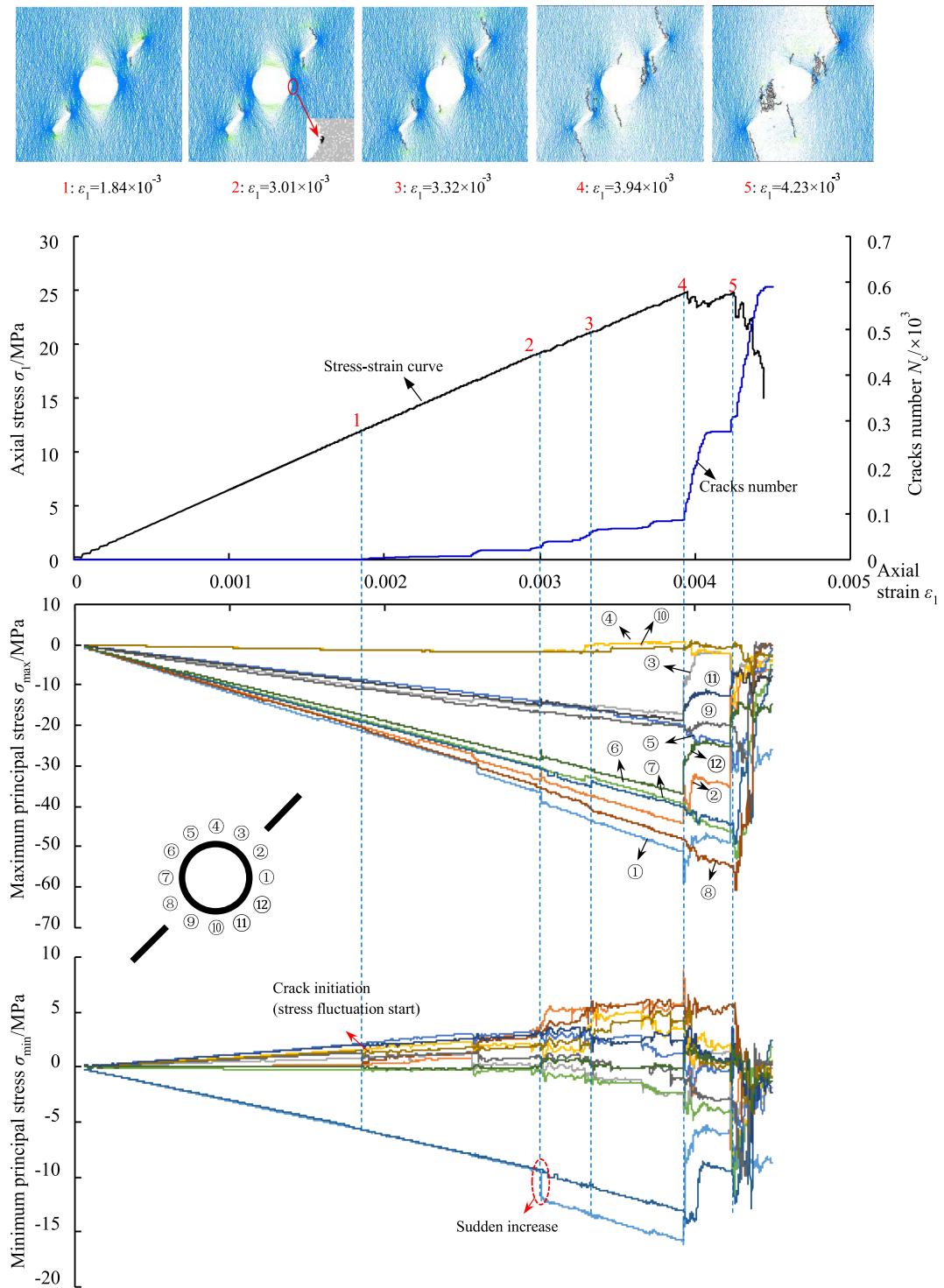
Figure 18. The stress-strain curve, cracking process and local principal stress evolution around the opening during the uniaxial loading process, \beta = 45^\circ .
