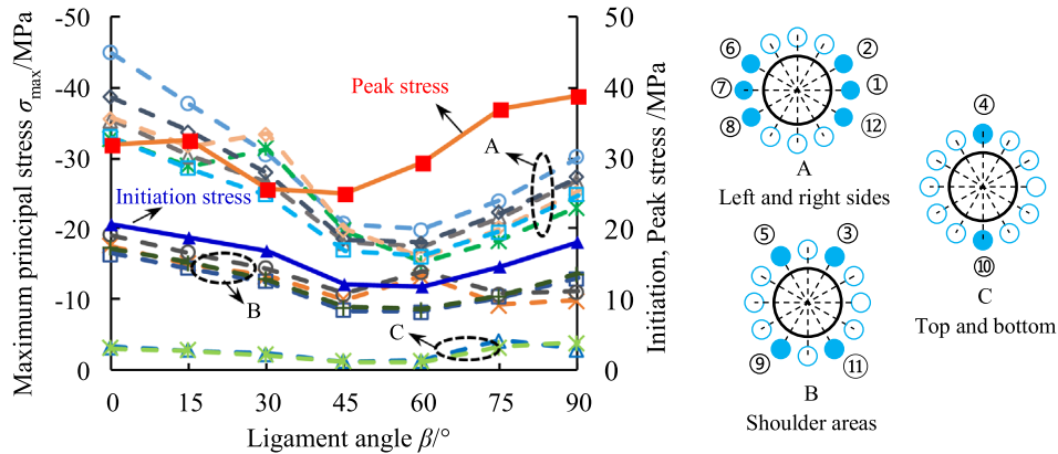
Figure 20. The relationship between local maximum principal stress around the opening and strength of H-J specimens.
