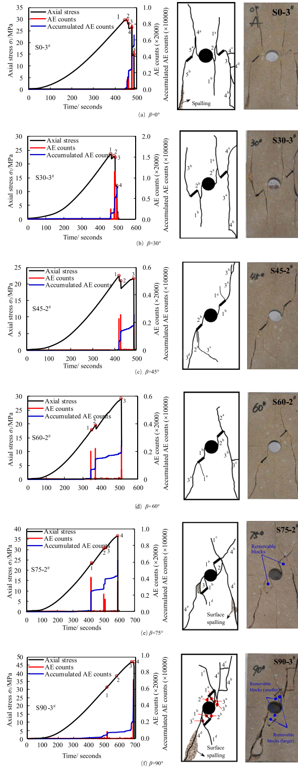
Figure 8. The axial stress, AE counts and cracking evolution sketch of H-J sandstone specimens with different ligament angle.
