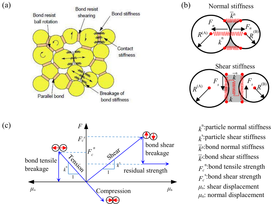
Figure 9. Bonded particle model (BPM) in PFC. (a) schematic representation of the bonded particle model [34]. (b) micro-scale properties of the bonded particle model [35]. (c) the mechanism of yielding bonds under normal and shear loads [35].
