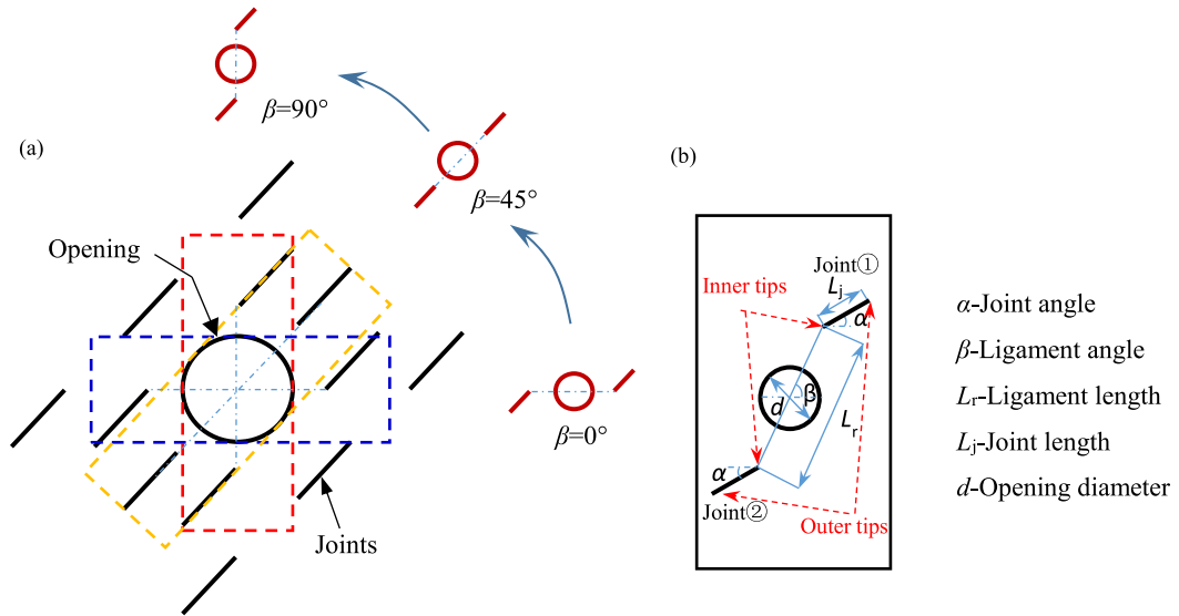
Figure 1. The relative position between the opening and surrounded non-persistent joints (a) and simplified research model in this study (b).
