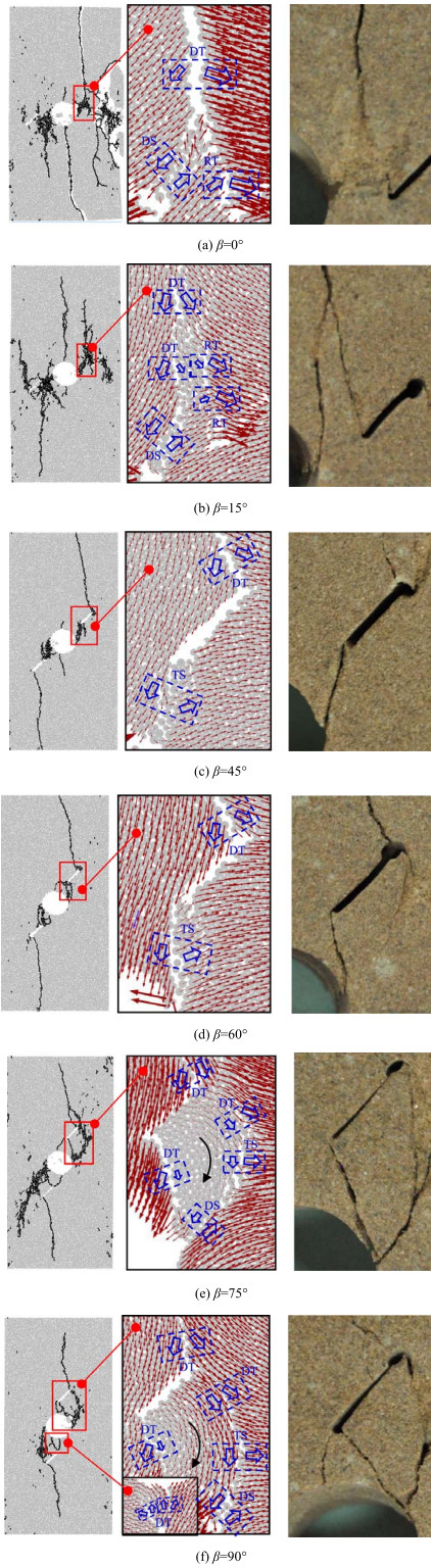
Figure 21. Local displacement fields of coalescence areas between the opening and joints.
