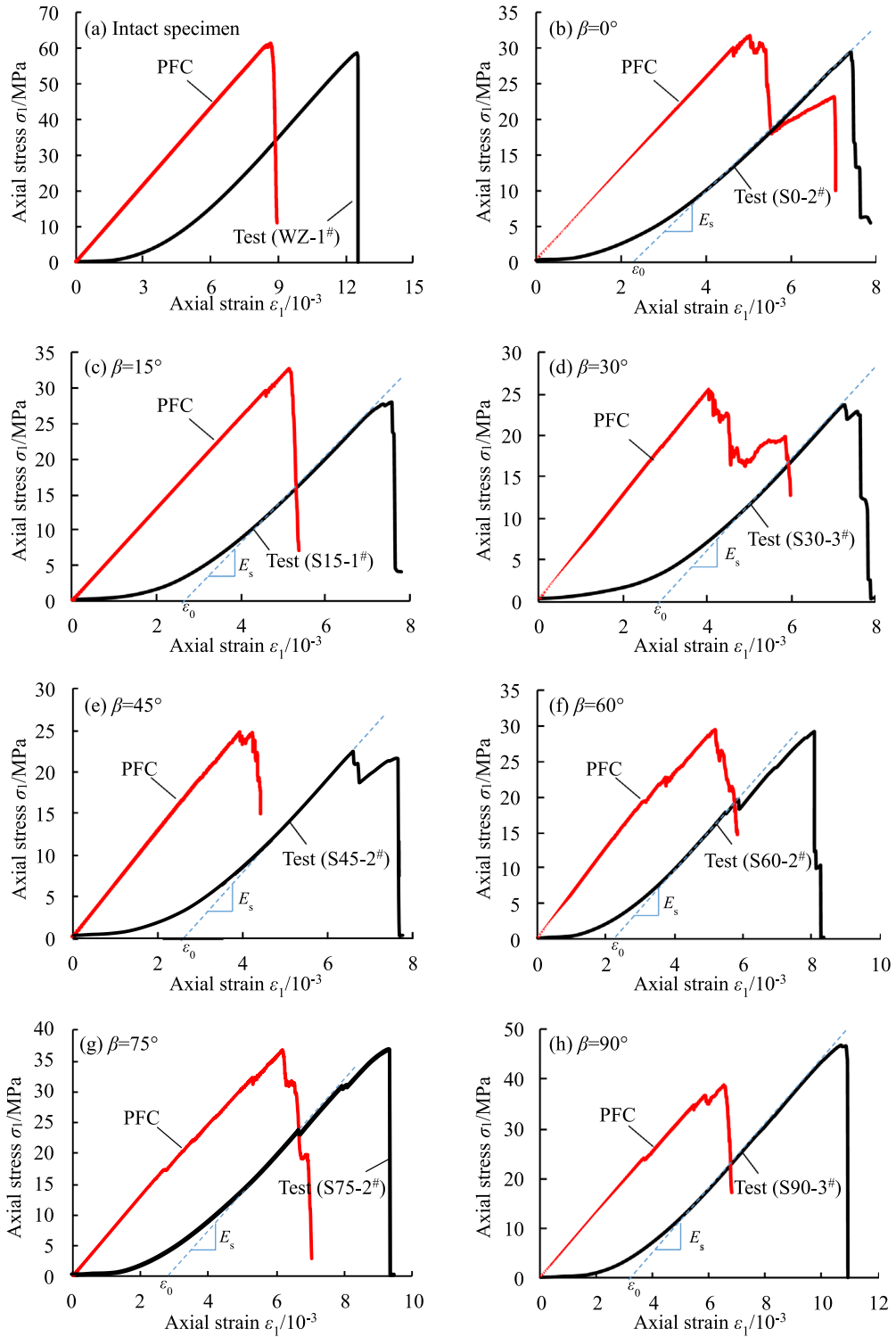
Figure 11. Comparison of stress-strain curves between laboratory tests and numerical simulation.
