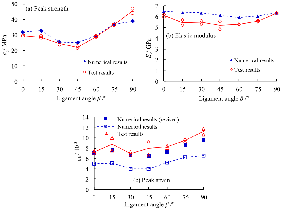
Figure 12. Comparison of strength and deformation parameters between laboratory tests and numerical simulation. (a) Peak strength. (b) Elastic modulus. (c) Peak strain.
