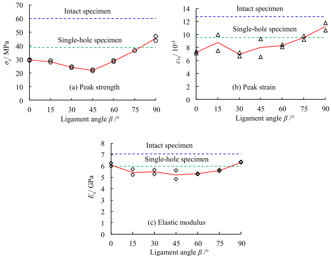
Figure 6. Influence of ligament angle on strength and deformation parameters of H-J sandstone specimens. (a) Peak strength. (b) Peak strain. (c) Elastic modulus.
