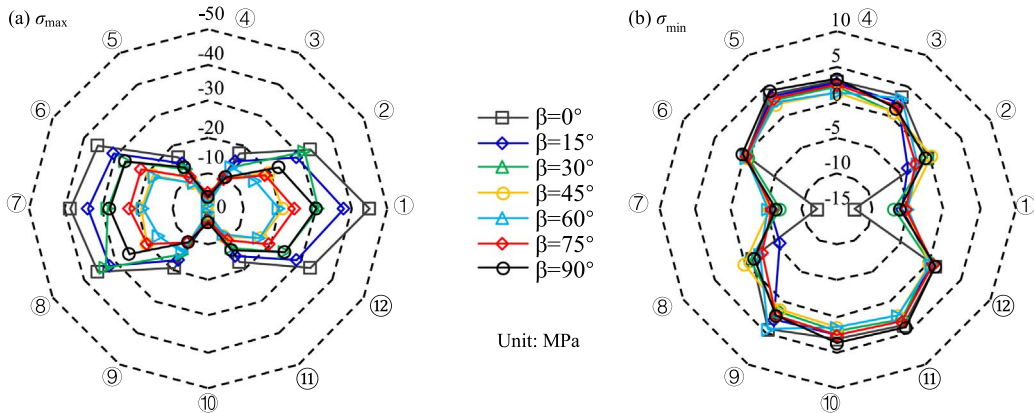
Figure 16. The principal stress distribution around a circular opening for H-J specimens with different ligament angle. (a) Maximum principal stress, \sigma_{\max} . (b) Minimum principal stress, \sigma_{\min} .
