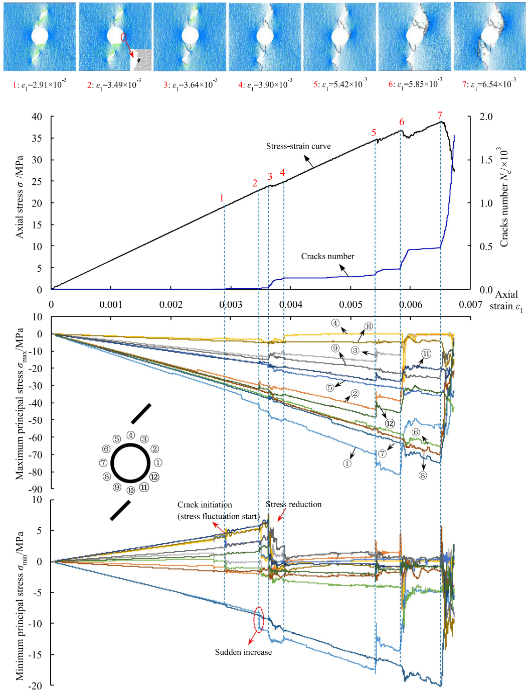
Figure 19. The stress-strain curve, cracking process and local principal stress evolution around the opening during the uniaxial loading process, \beta = 90^\circ .
