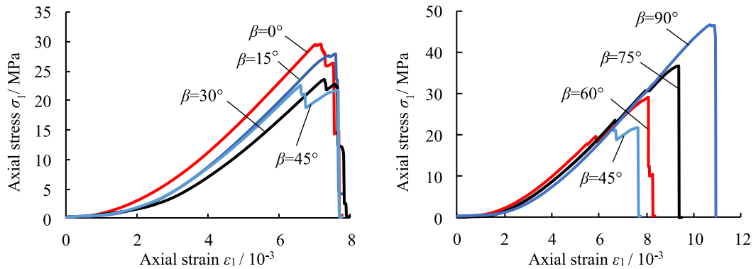
Figure 5. Effect of ligament angle on stress-strain curves of H-J sandstone specimens.
