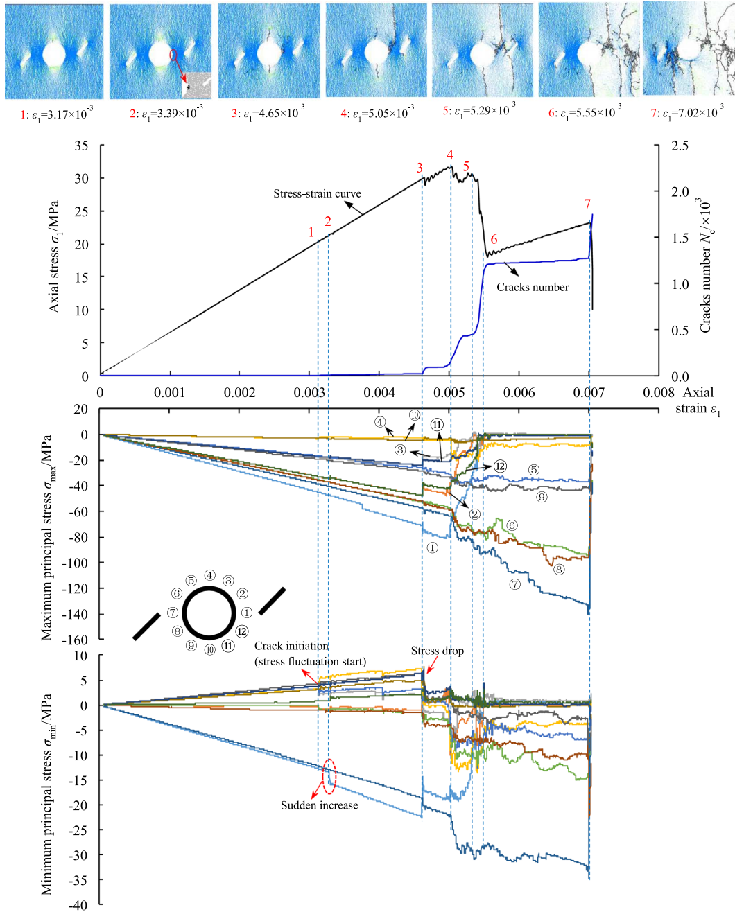
Figure 17. The stress-strain curve, cracking process and local principal stress evolution around the opening during the uniaxial loading process, \beta = 0^\circ .
