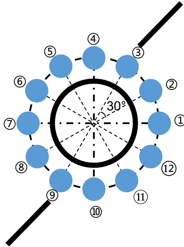
Figure 15. The arrangement of measurement spheres around circular opening in H-J specimens.
