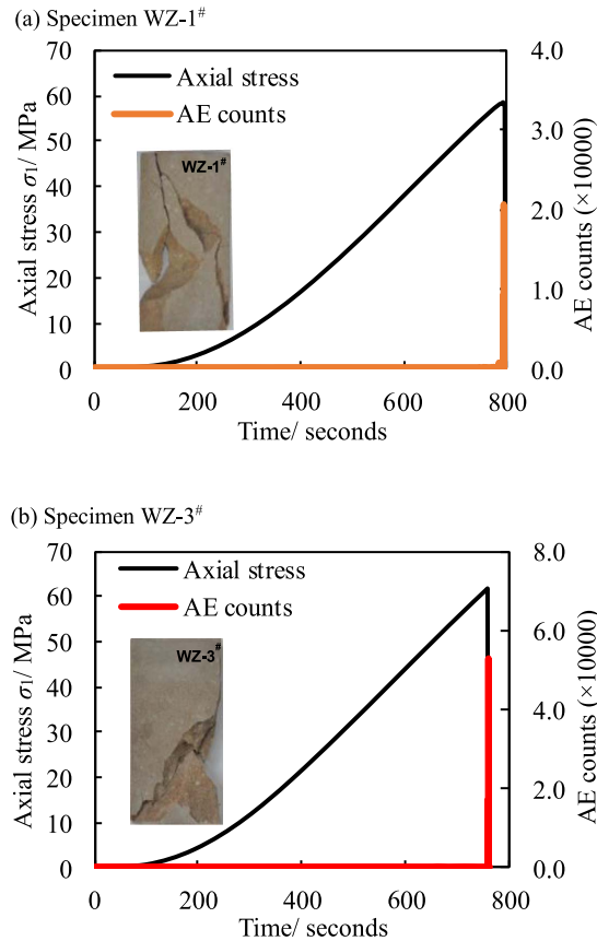
Figure 3. Experimental results of intact sandstone specimens under uniaxial compression. (a) Specimen WZ-1#. (b) Specimen WZ-3#.
