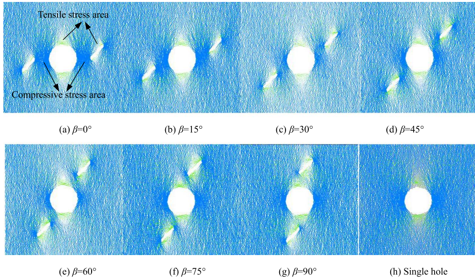
Figure 14. The local stress field around opening and joints just before cracks initiation.
