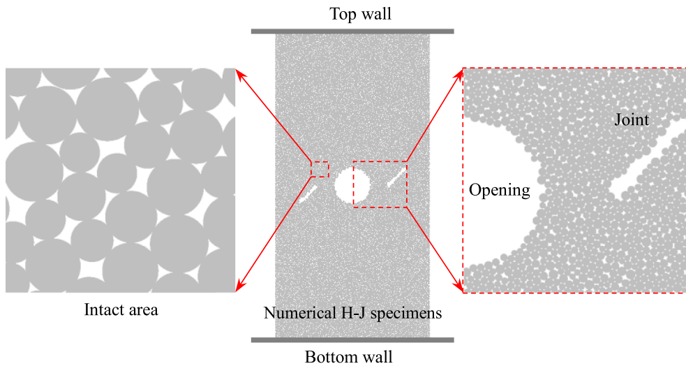
Figure 10. The established numerical H-J specimens using PFC 2D .
