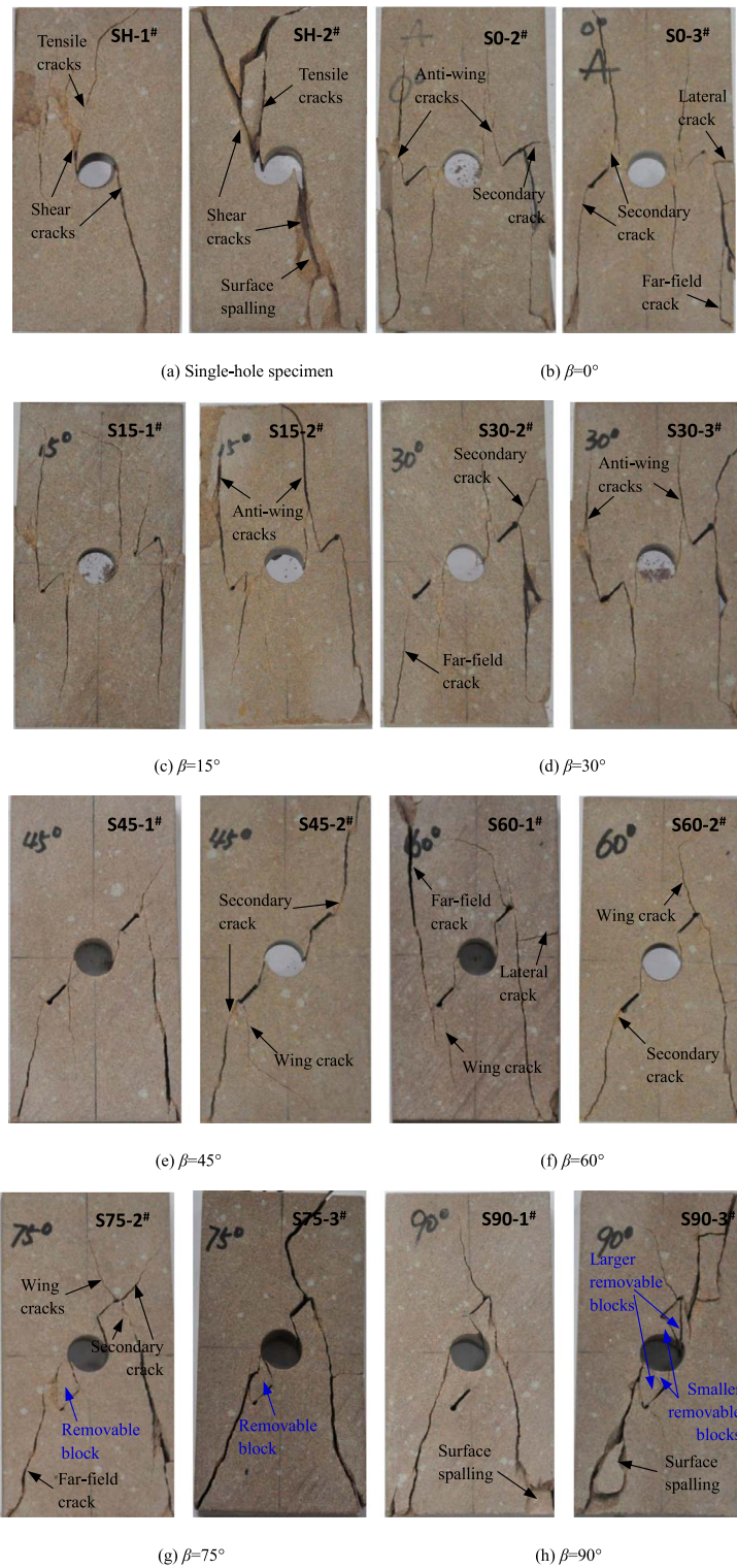
Figure 7. Ultimate failure modes of single-hole specimens and H-J specimens with different ligament angles.
