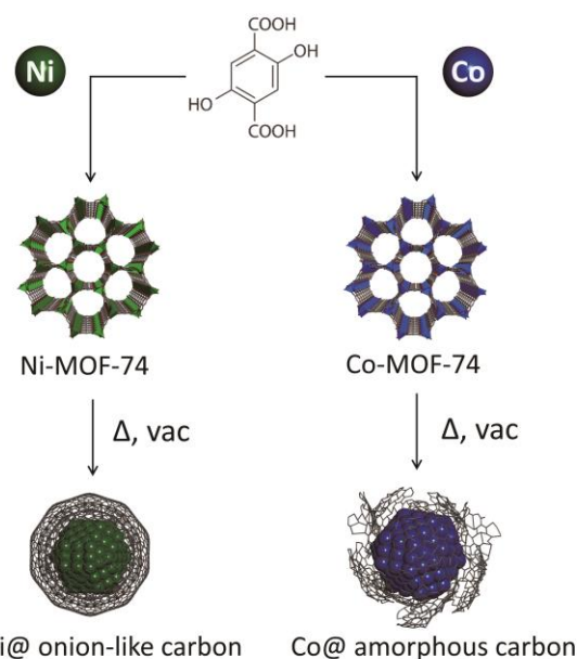
Scheme 1 Synthesis of Ni@onion-like carbon and Co @amorphous carbon.
