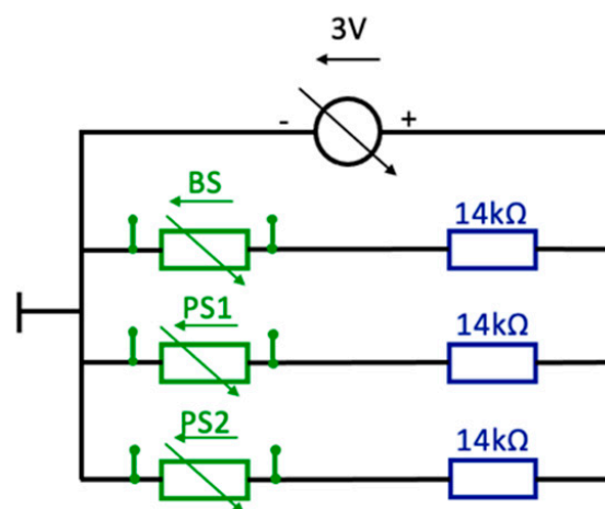
Figure 10. Schematic of the circuit for evaluating the sensors with three 14 kΩ resistors, voltage source, the two pressure sensors (PS1 and PS2), and the bending sensor (BS).
