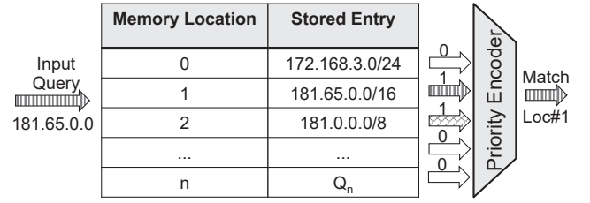
Fig. 1: Network search operation in TCAM.
