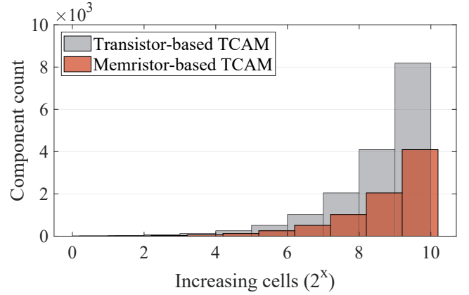
Fig. 12: Packing density of memristor-based TCAM cells.
