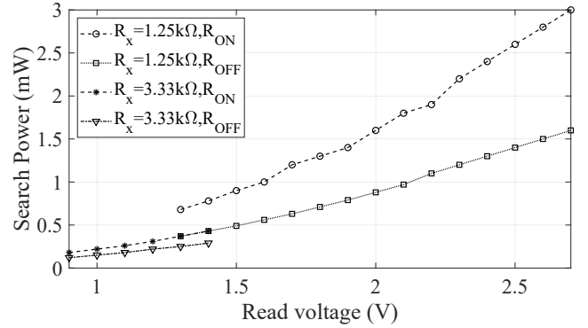
Fig. 10: Search power trends with variation in R_x .
