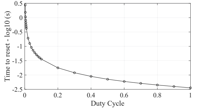
Fig. 11: Reset time of TCAMM CogniGron .
