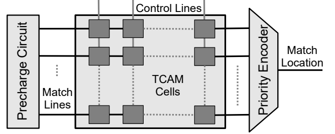
Fig. 2: Architecture of TCAM memory.
