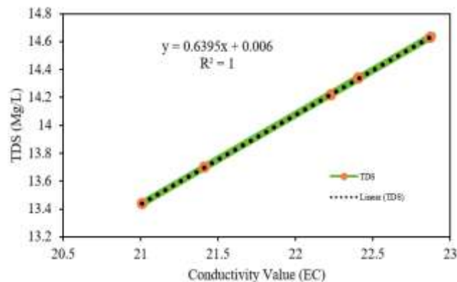
Figure 6. Conductivity graph of meatball samples
