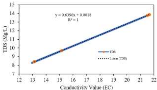
Figure 9. The correlation between EC and TDS
