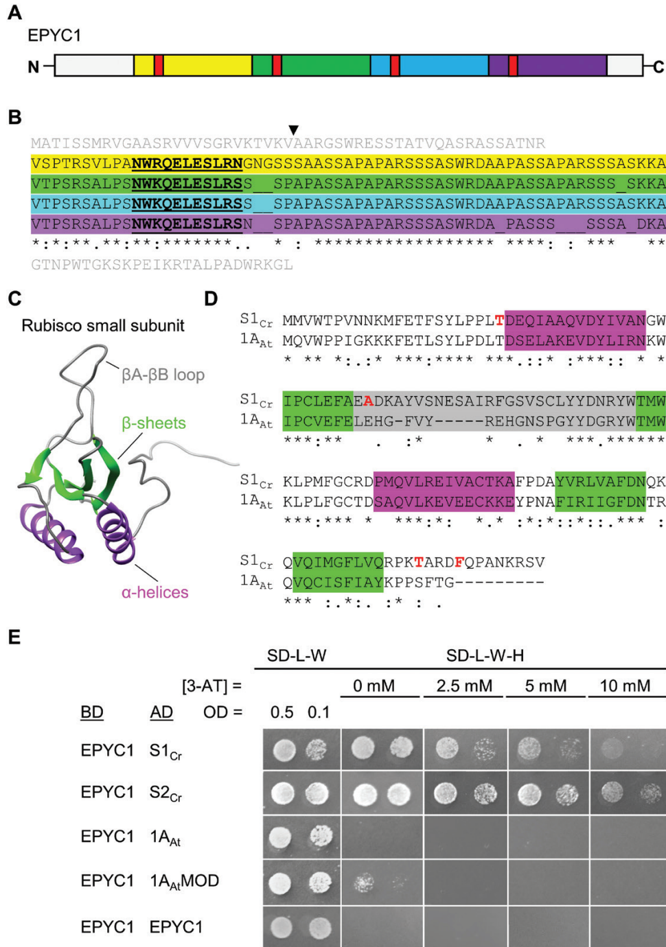
Fig. 1. EPYC1 interacts with the Rubisco small subunit. (A and B) EPYC1 consists of four near identical repeat regions (highlighted in yellow, green, blue, and purple), each containing a predicted \alpha -helix (red, underlined). The putative cleavage site of the chloroplastic transit peptide between 26 (V) and 27 (A) is indicated. The N- and C- termini are shown in grey. (C) The predicted model of the small subunit of Rubisco (SSU; 1A At shown) has similar features in algae and higher plants, including four \beta -sheet (green) and two \alpha -helical (purple) regions. (D) Amino acid alignments of mature Arabidopsis SSU 1A (1A At ) and Chlamydomonas SSU 1 (S1 Cr ). Residues in red indicate the four amino acids that differ between the two Chlamydomonas SSUs, S1 Cr and S2 Cr (T/S, A/S, T/S, F/W). (E) Yeast two-hybrid interactions with EPYC1. Interaction strength is demonstrated by growth on increasing concentrations of the inhibitor 3-AT. Abbreviations: 3-AT, 3-amino-1,2,4-triazole; BD, binding domain; AD, activation domain; 1A At MOD, modified 1A At carrying the two \alpha -helical regions from Chlamydomonas; SD-L-W, yeast synthetic minimal medium (SD medium) lacking leucine (L) and tryptophan (W); SD-L-W-H, SD medium lacking L, W, and histidine (H). See Supplementary Fig. S1 for Y2H additional controls.
